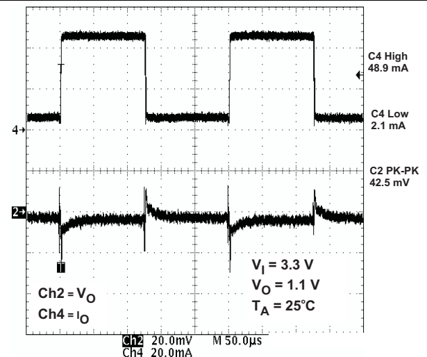
Figure 27. LDO1 Load Transient Response
