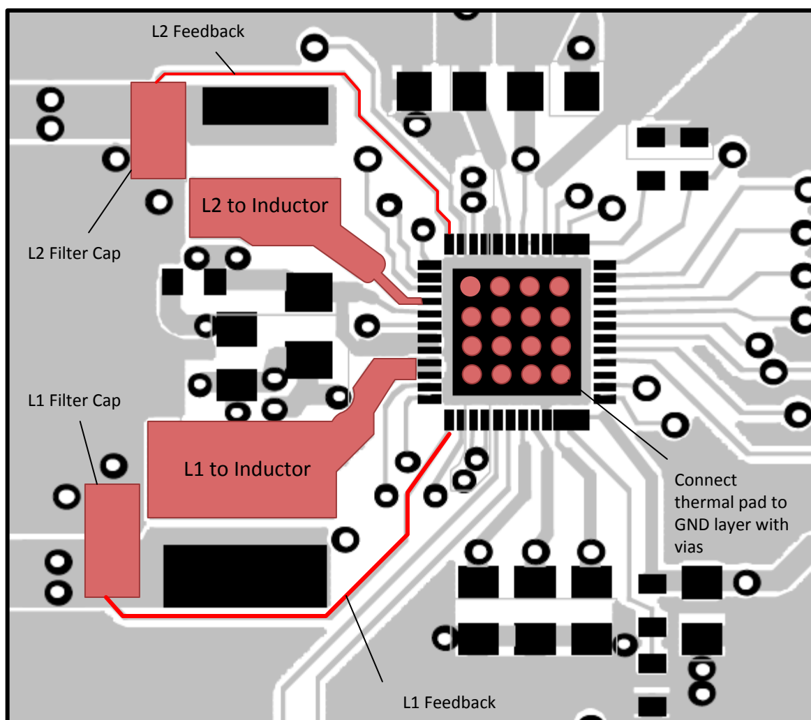
Figure 46. EVM Layout
