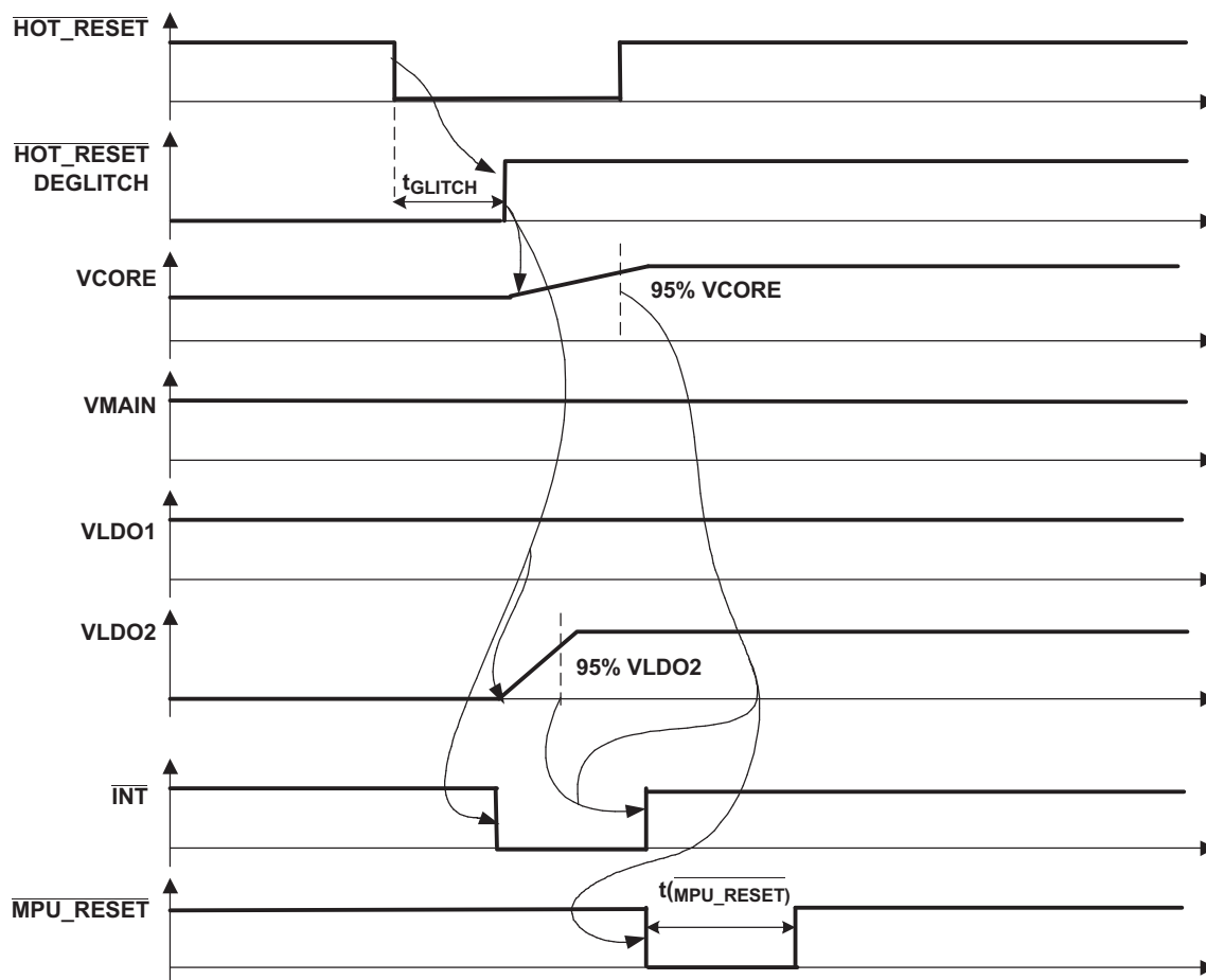
Figure 35. State 3 to State 2 Transition ( \overline{HOT\_RESET} Activated, See Interrupt Management for \overline{INT} Behavior)
