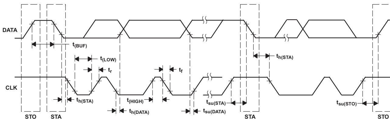
Figure 41. Serial Interface Timing Diagram
