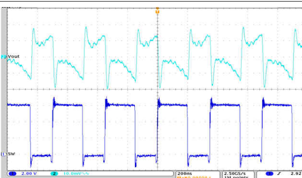
Figure 9-77. Output Voltage Ripple
