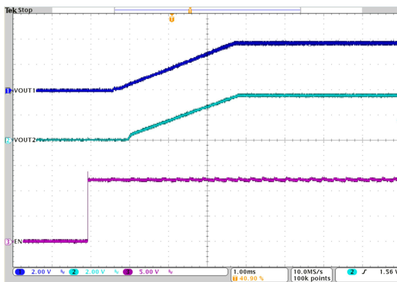
Figure 9-84. Tracking
