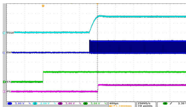
Figure 9-65. Start-Up Timing
