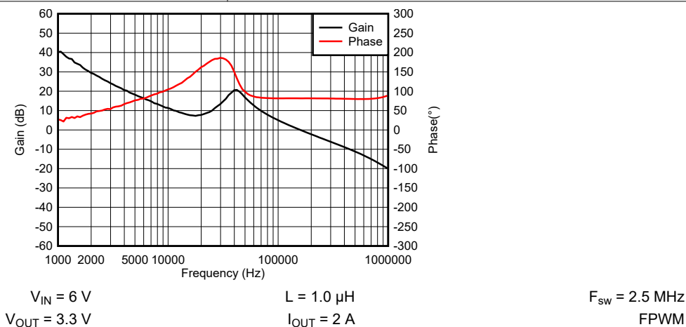
Figure 9-80. Bode Plot
