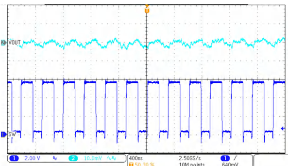
Figure 9-77. Output Voltage Ripple
