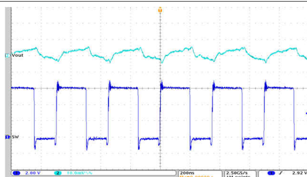
Figure 9-76. Output Voltage Ripple
