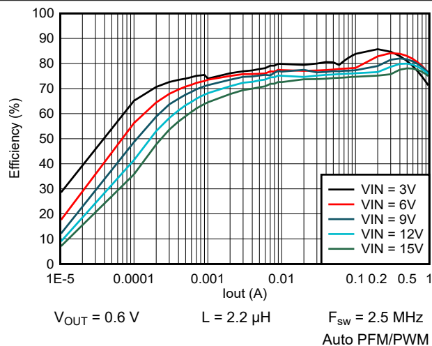
Figure 9-50. Efficiency vs Output Current
