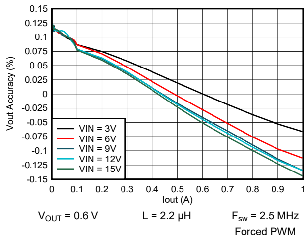
Figure 9-55. Output Voltage vs Output Current
