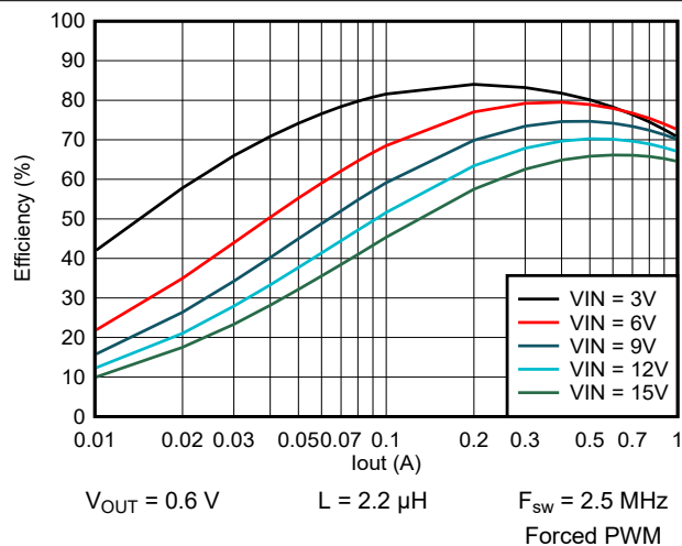
Figure 9-51. Efficiency vs Output Current
