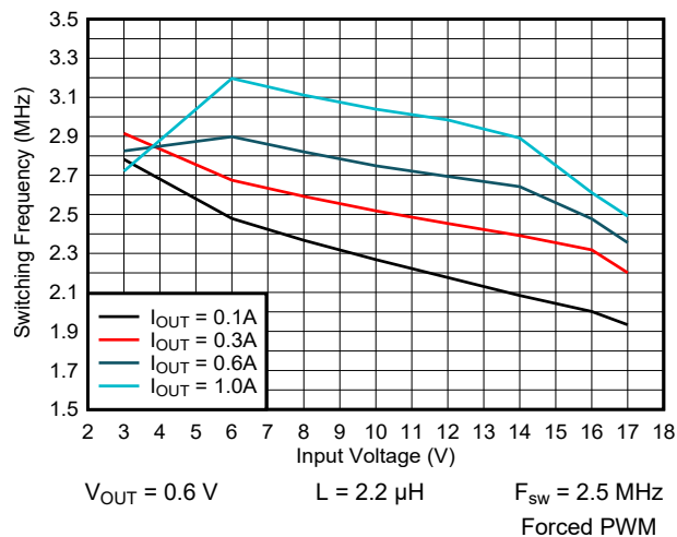
Figure 9-53. Switching Frequency vs Input Voltage
