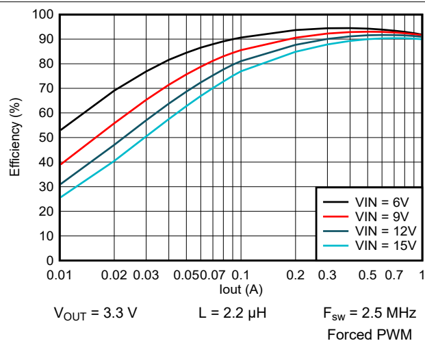
Figure 9-15. Efficiency vs Output Current
