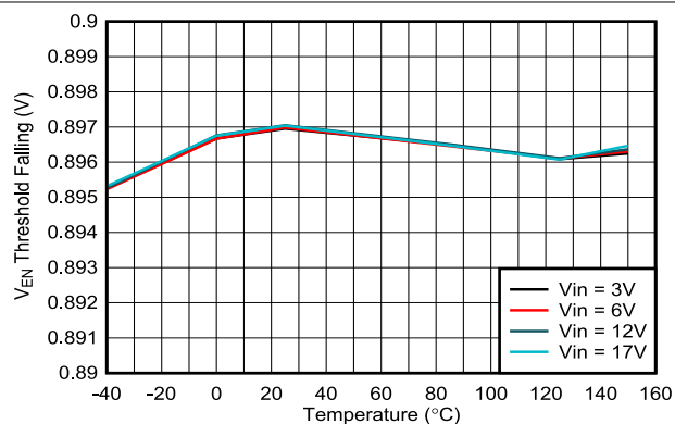
Figure 7-18. Precision Enable Threshold vs Temperature
