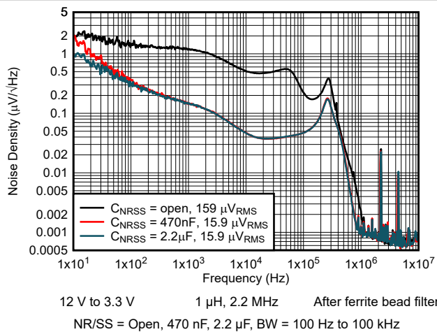
Figure 5-18. Output Noise Density vs Frequency
