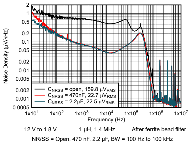
Figure 5-16. Output Noise Density vs Frequency
