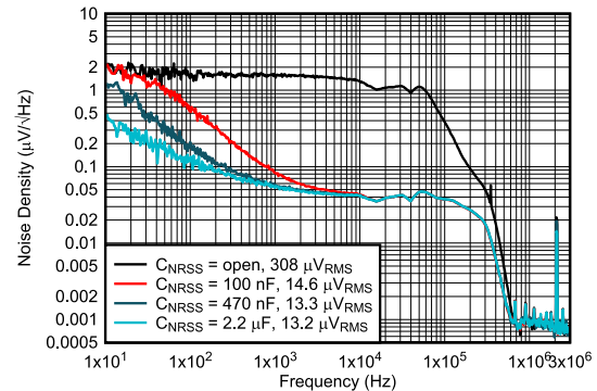
Figure 6-40. Output Noise Density vs Frequency
