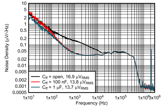
Figure 6-38. Output Noise Density vs Frequency
