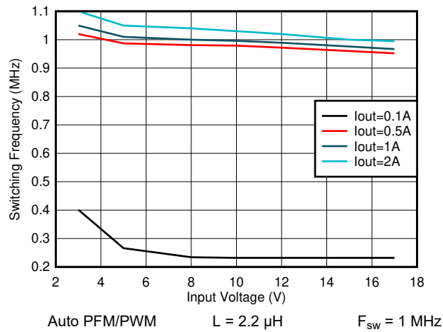
Figure 8-31. Switching Frequency vs Input Voltage V_{OUT} = 1.8 V
