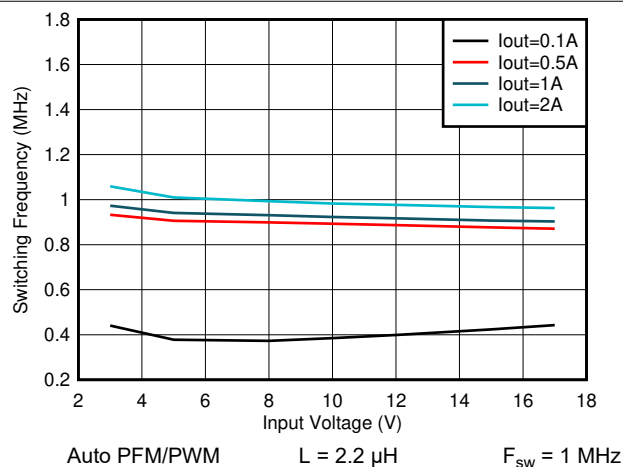
Figure 8-35. Switching Frequency vs Input Voltage V_{OUT} = 1.2 V
