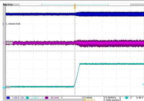
V_{IN} = 6\text{ V to 11 V} 2.5 MHz Auto I_O = 1\text{ A} PFM/PWM V_{OUT} = 3.3\text{ V} T_A = 25^\circ\text{C}
