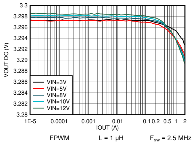
Figure 8-39. Output Voltage vs Output Current V_{\text{OUT}} = 3.3 \text{ V}
