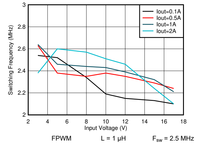
Figure 8-34. Switching Frequency vs Input Voltage V_{OUT} = 1.8 V
