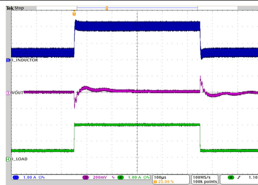
V_{IN} = 12\text{ V} 2.5 MHz Auto I_O = 500\text{ mA to 2 A to 500 mA} PFM/PWM V_{OUT} = 3.3\text{ V} T_A = 25^\circ\text{C}
