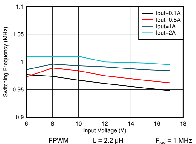
Figure 8-24. Switching Frequency vs Input Voltage V OUT = 5 V
