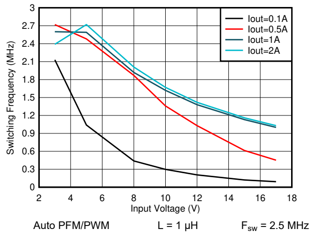
Figure 8-33. Switching Frequency vs Input Voltage V_{OUT} = 1.8 V
