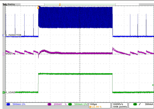
V_{IN} = 12\text{ V} 1 MHz Auto I_O = 5\text{ mA to 1 A to 5 mA} PFM/PWM V_{OUT} = 3.3\text{ V} T_A = 25^\circ\text{C}
