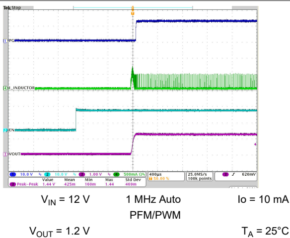
Figure 8-41. Start-up Timing
