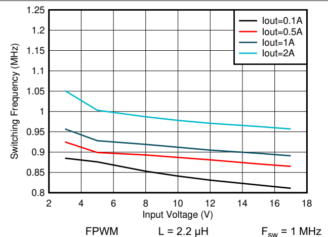
Figure 8-36. Switching Frequency vs Input Voltage V_{OUT} = 1.2 V
