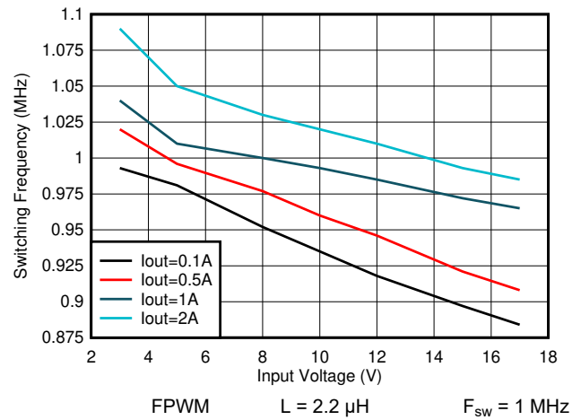
Figure 8-32. Switching Frequency vs Input Voltage V_{OUT} = 1.8 V
