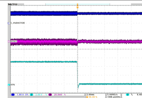
V_{IN} = 11\text{ V to 6 V} 2.5 MHz Auto I_O = 1\text{ A} PFM/PWM V_{OUT} = 3.3\text{ V} T_A = 25^\circ\text{C}
