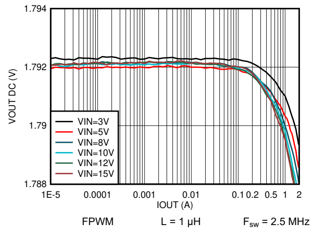
Figure 8-40. Output Voltage vs Output Current V_{\text{OUT}} = 1.8 \text{ V}
