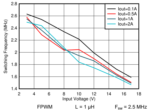
Figure 8-38. Switching Frequency vs Input Voltage V_{\text{OUT}} = 1.2 \text{ V}
