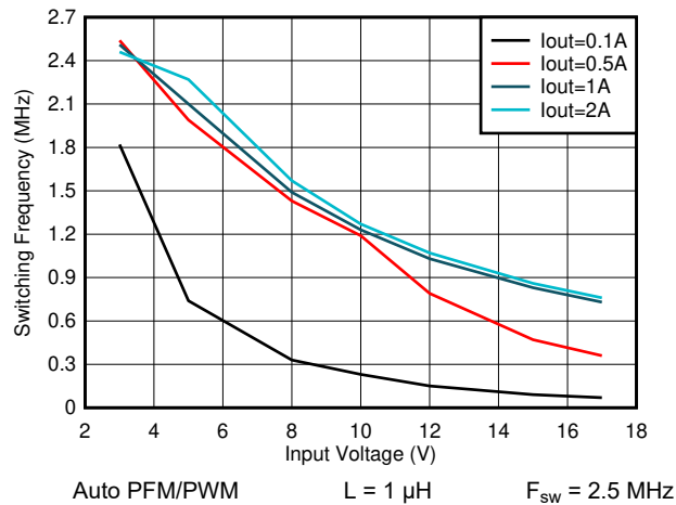
Figure 8-37. Switching Frequency vs Input Voltage V_{\text{OUT}} = 1.2 \text{ V}
