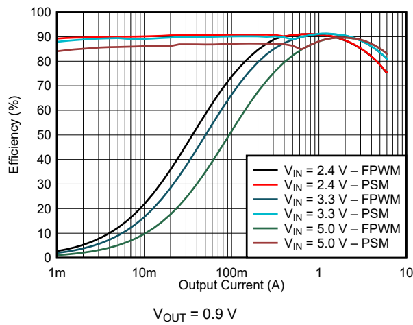
Figure 9-4. Efficiency
