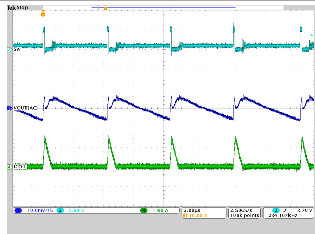
Figure 9-15. Switching Frequency
