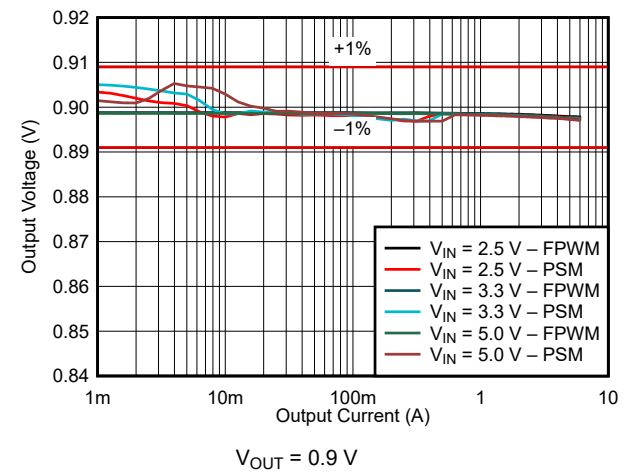
Figure 9-5. Load Regulation
