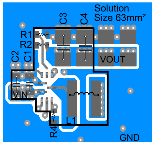
Figure 11-1. Layout Example
