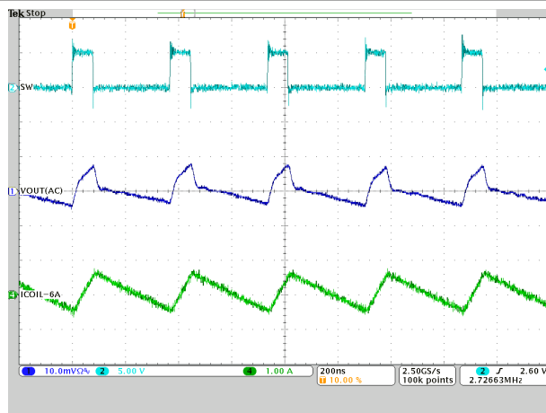
Figure 9-14. Switching Frequency
