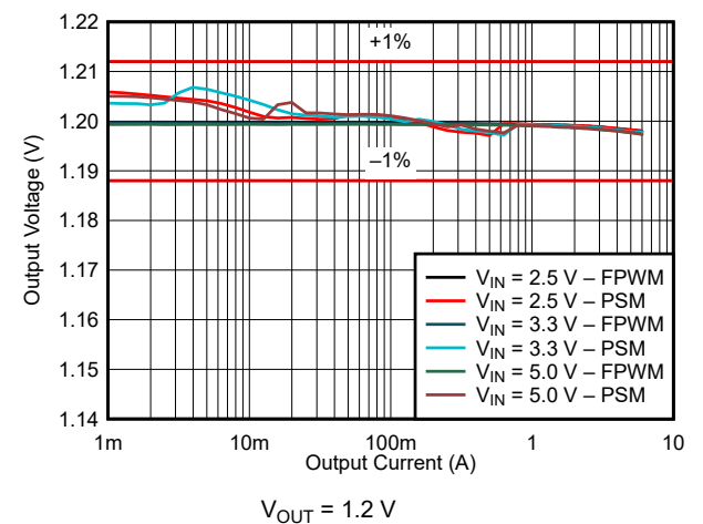
Figure 9-7. Load Regulation
