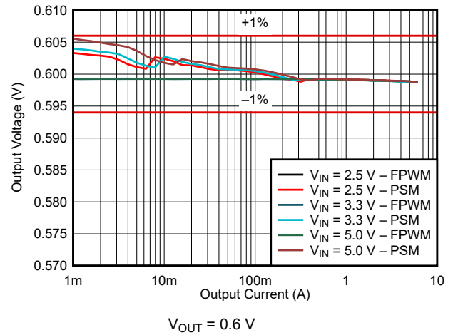
Figure 9-3. Load Regulation
