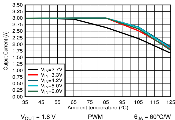
Figure 9-20. Output Current vs Ambient Temperature
