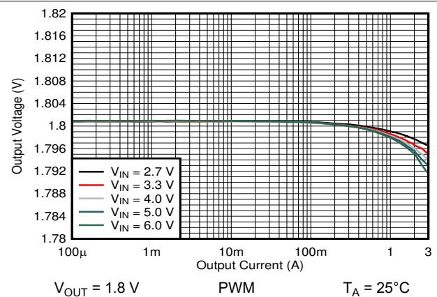
Figure 9-13. Output Voltage vs Output Current
