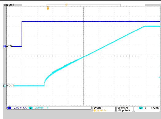
Figure 9-52. Start-Up Timing
