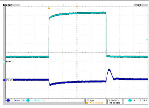
Figure 10-31. Load Transient Response
