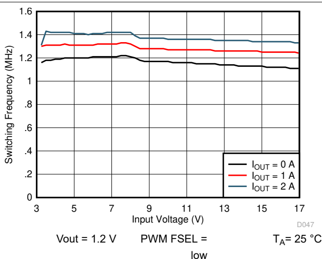
Figure 10-67. Switching Frequency vs Input Voltage
