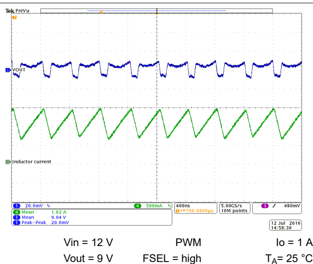
Figure 10-65. Output Voltage Ripple
