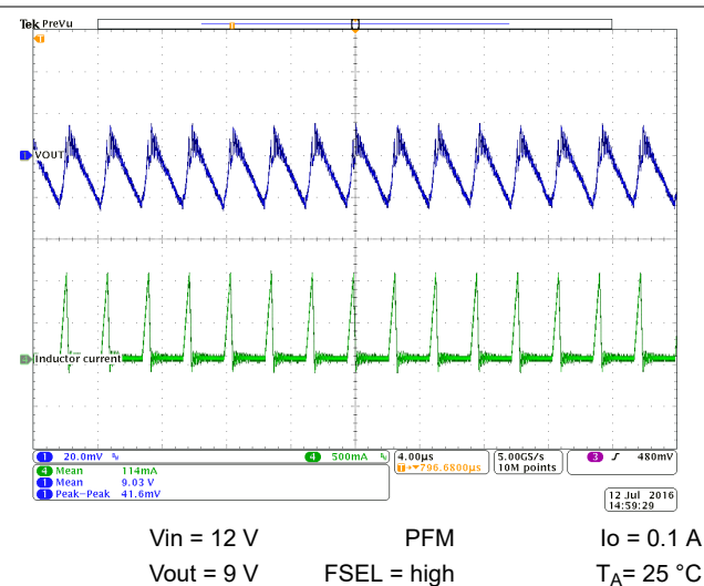
Figure 10-64. Output Voltage Ripple
