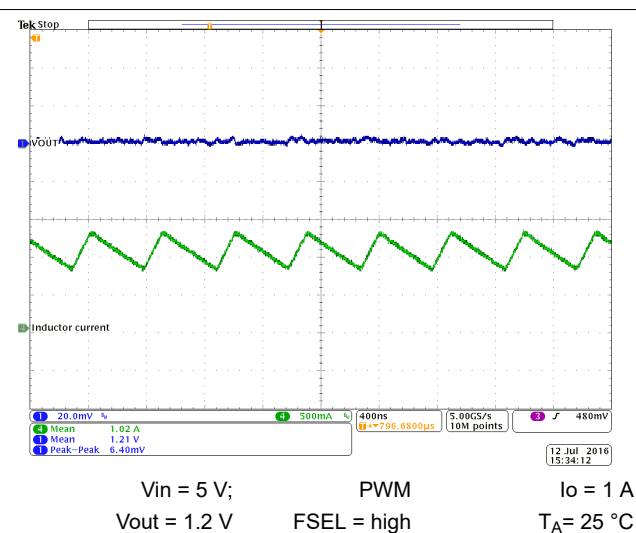
Figure 10-37. Output Voltage Ripple
