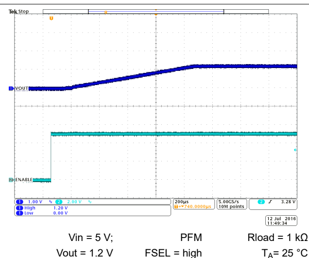
Figure 10-35. Start-Up Timing
