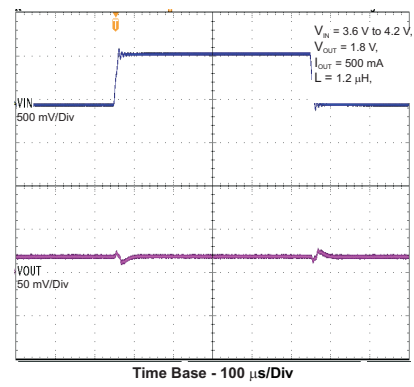
Time Base - 100µs/Div Figure 20. Line Transient Response PWM Mode
