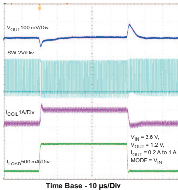
Time Base - 10µs/Div Figure 17. Load Transient Response PWM Mode 0.2 A to 1 A
