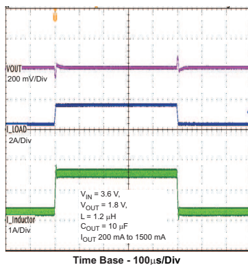
Time Base - 100µs/Div Figure 19. Load Transient Response 200 mA to 1500 mA
