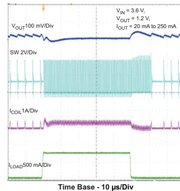
Time Base - 10µs/Div Figure 18. Load Transient PFM Mode 20 mA to 250 mA
