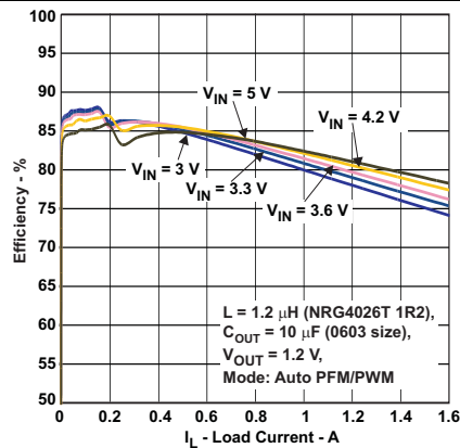
Figure 9. Efficiency vs Load Current V OUT = 1.2 V, Auto PFM/PWM Mode, Linear Scale
