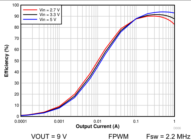
Figure 6-4. 9 V_{OUT} Efficiency vs Output Current
