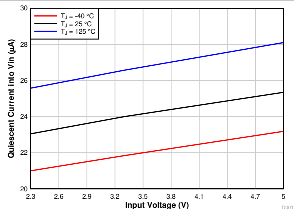
Figure 6-6. Quiescent Current into V_{IN} vs Input Voltage
