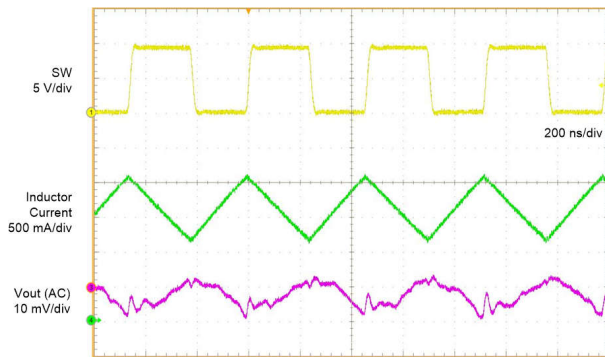
Figure 8-5. Switching Waveform V_{\text{IN}} = 5\text{ V} , V_{\text{OUT}} = 9\text{ V} , I_{\text{OUT}} = 800\text{ mA} , FPWM
