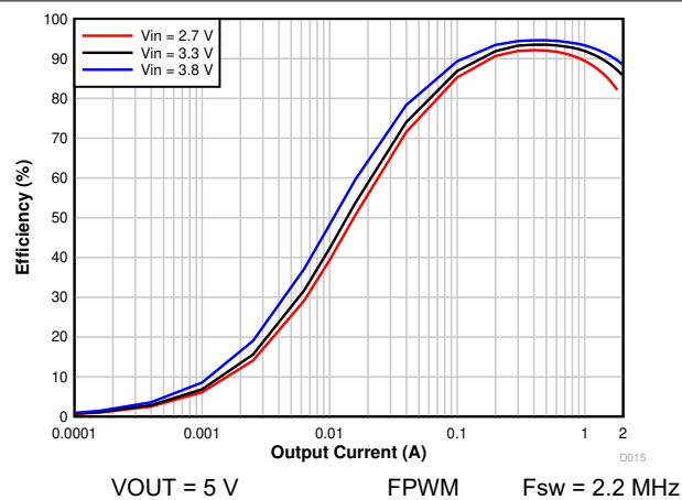
Figure 6-2. 5 V_{OUT} Efficiency vs Output Current
