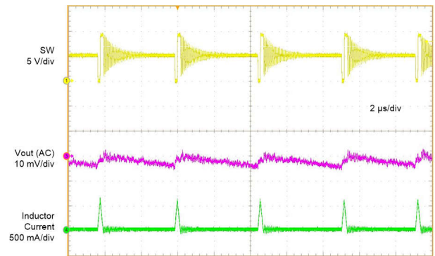
Figure 8-6. Switching Waveform V_{\text{IN}} = 5\text{ V} , V_{\text{OUT}} = 9\text{ V} , I_{\text{OUT}} = 0\text{ mA} , Auto PFM
