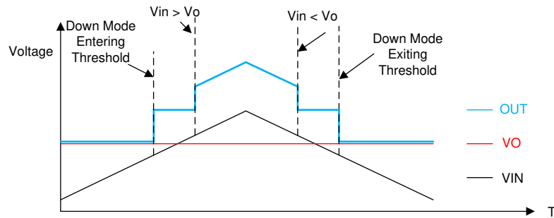
Figure 7-1. Down Mode
