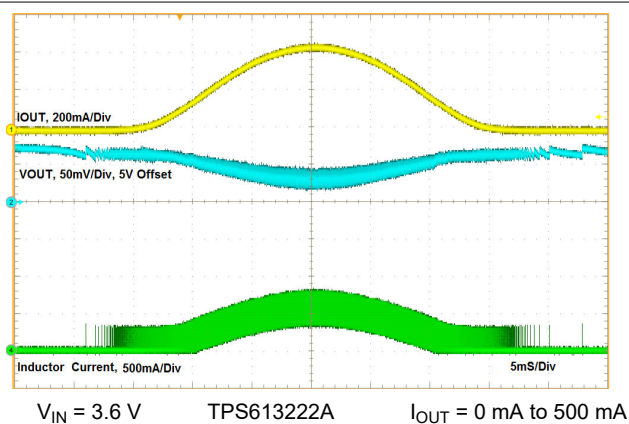
Figure 8-17. Load Regulation
