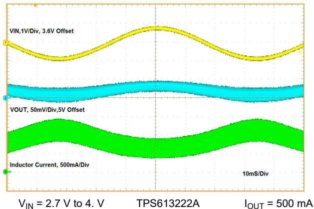
Figure 8-15. Line Regulation
