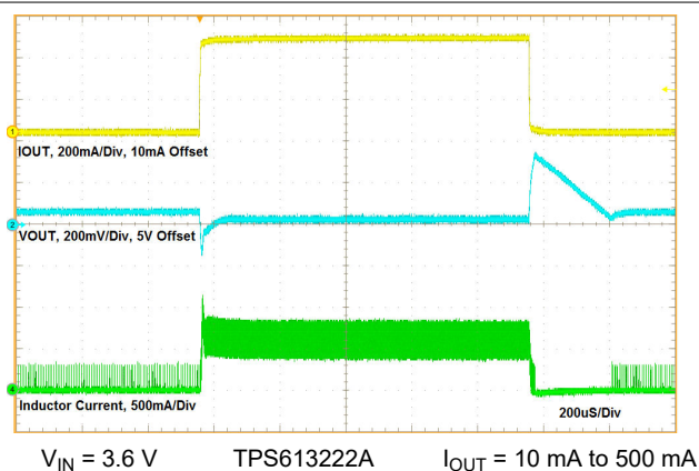
Figure 8-16. Load Transient
