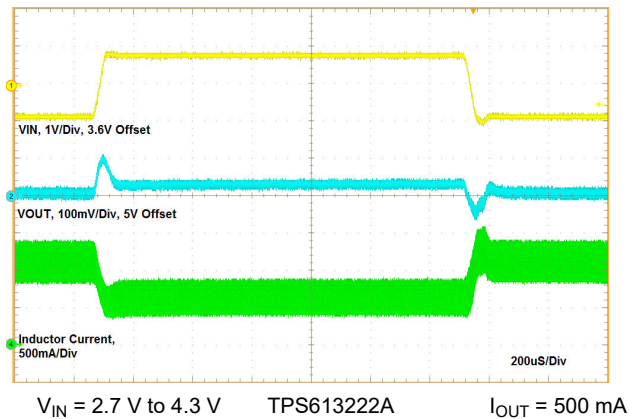
Figure 8-14. Line Transient
