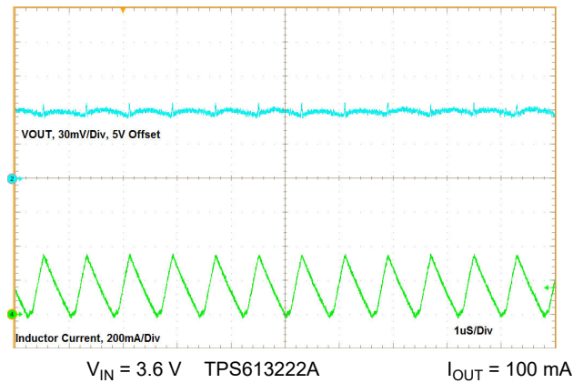
Figure 8-11. Switching Waveform at Heavy Load
