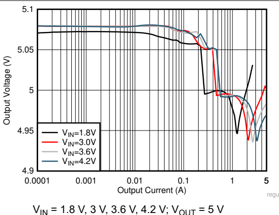
Figure 6-5. Load Regulation in Auto PFM
