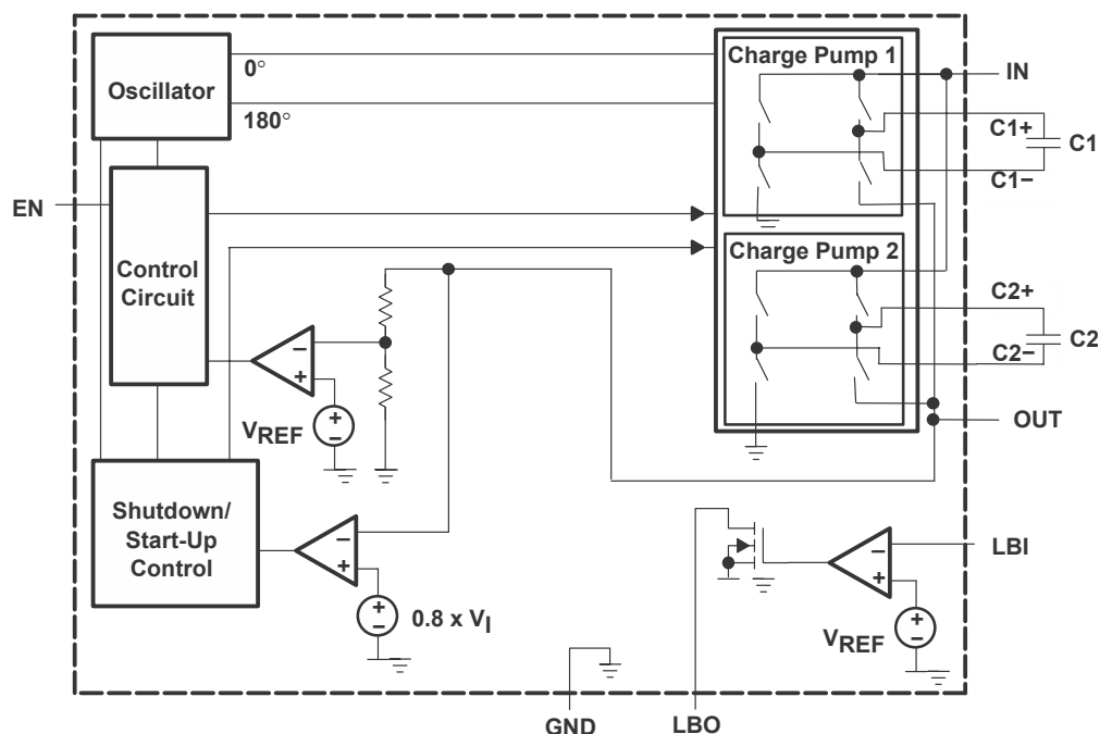
Figure 8-2. TPS60204 With Low-Battery Detector
