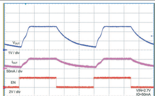
Figure 20. Enable / Disable V IN = 2.7 V, I O = 50 mA
