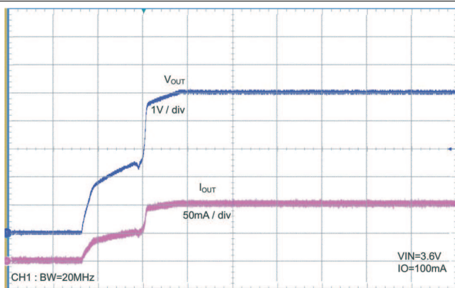
Figure 19. Power On V IN = 3.6 V, I O = 100 mA
