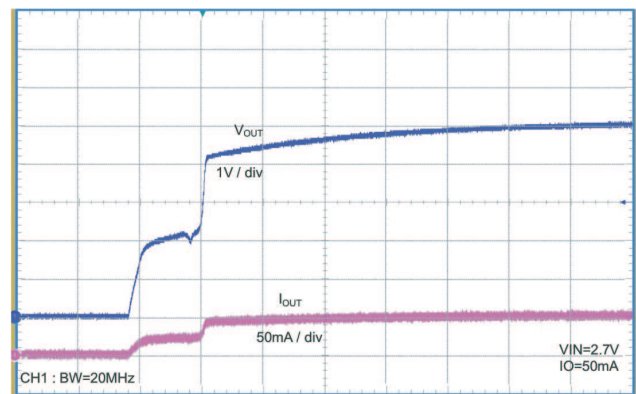
Figure 18. Power On V IN = 2.7 V, I O = 50 mA
