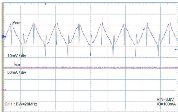
Figure 17. Output Ripple (Normal Mode) V IN = 3.6 V, I O = 100 mA
