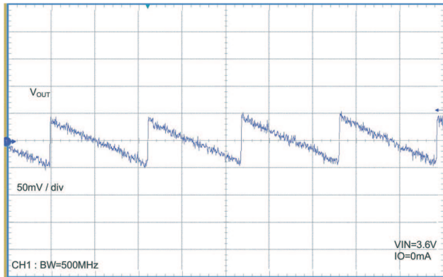
Figure 15. Output Ripple Voltage (Skip Mode) V IN = 3.6 V, I O = 0 mA
