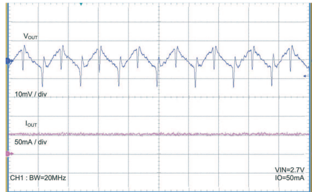
Figure 16. Output Ripple Voltage (Normal Mode) V IN = 2.7 V, I O = 50 mA
