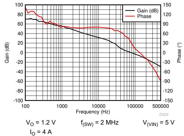
Figure 8-13. Closed-Loop Response
