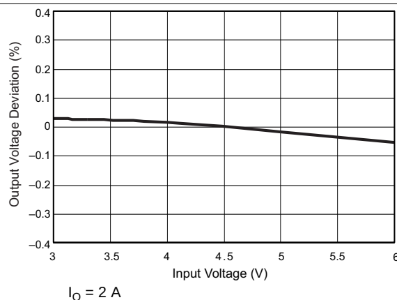
Figure 48. Regulation versus Input Voltage
