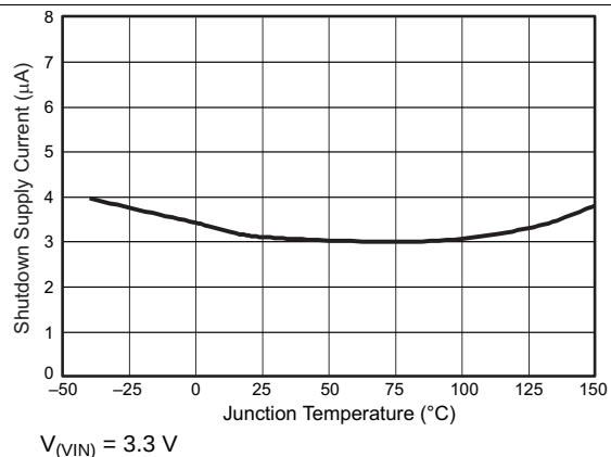
Figure 14. Shutdown Supply Current versus Temperature
