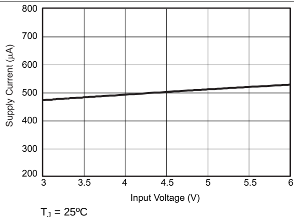
Figure 15. Shutdown Supply Current versus Input Voltage
