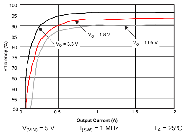
Figure 38. Efficiency versus Load Current 1 MHz, 5 VIN, T_A = 25^{\circ}\text{C}
