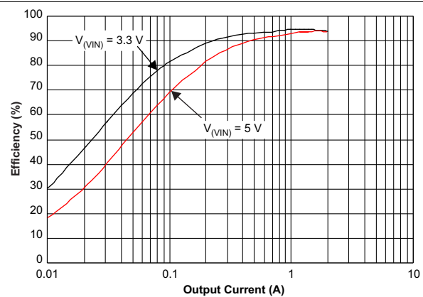
Figure 36. Efficiency versus Load Current
