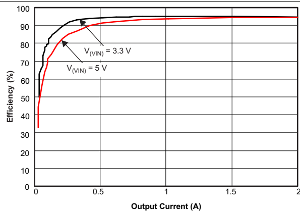
Figure 35. Efficiency versus Load Current
