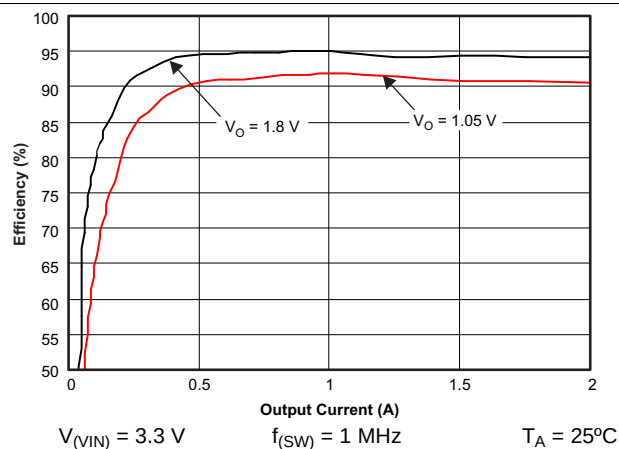
Figure 37. Efficiency versus Load Current 1 MHz, 3.3 VIN, T_A = 25^{\circ}\text{C}
