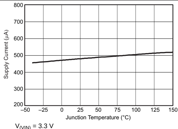
Figure 14. Shutdown Supply Current versus Temperature
