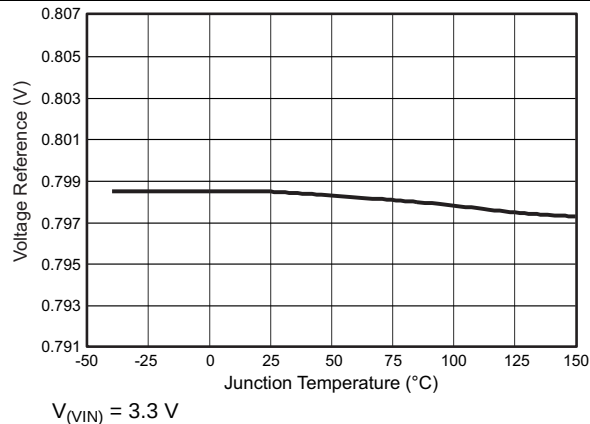
Figure 4. Voltage Reference versus Temperature
