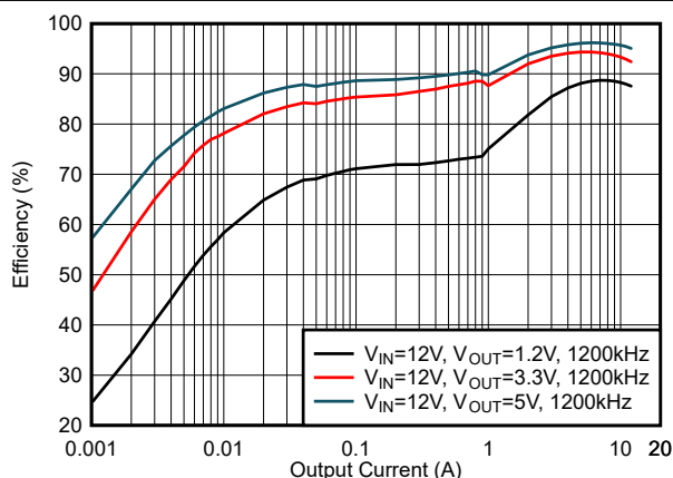
Figure 6-21. Efficiency, DCM Mode, f_{sw} = 1200\text{ kHz}
