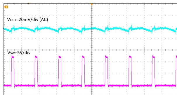
Figure 8-5. Output Voltage Ripple, I_{OUT} = 12\text{ A} , Time = 1 \mu\text{S/div}
