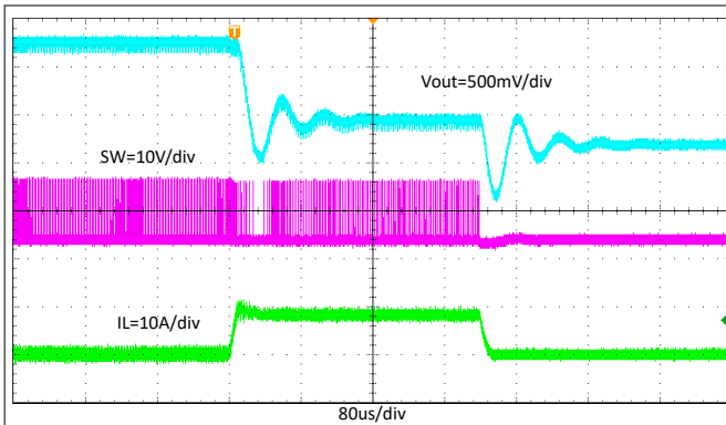
Figure 8-20. TPS566247 Normal Operation to Output Hard Short
