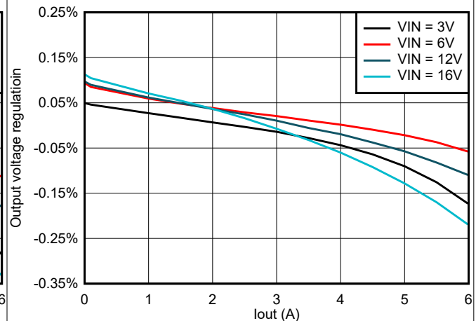
Figure 8-5. TPS566247 Load Regulation vs Loading
