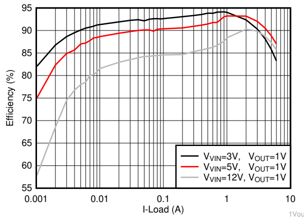
Figure 7-2. TPS566231 Efficiency Curve
