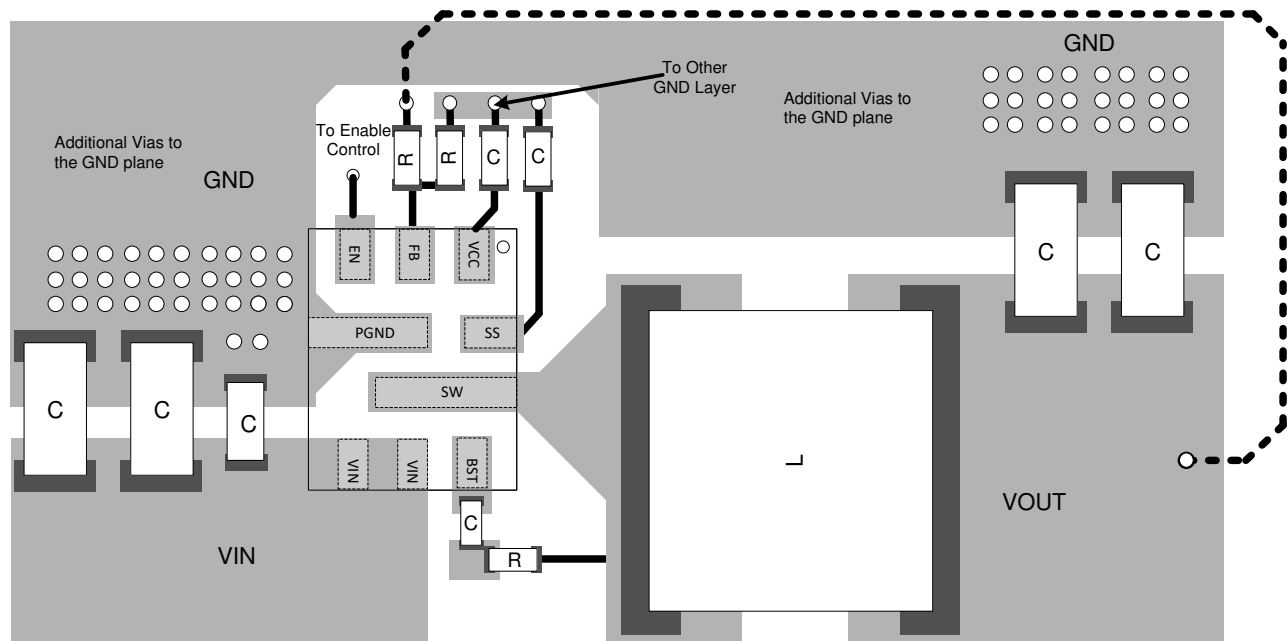
Figure 7-26. Top-Layer Layout
