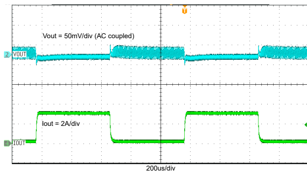
Figure 8-12. TPS563252 Transient Response with 0.1 A to 3 A
