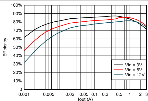
Figure 6-11. TPS563252 Efficiency at 0.6 V_{OUT} with a 0.68- \mu\text{H} Inductor
