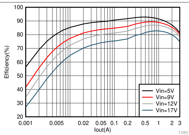
Figure 8. TPS563231 V_{OUT} = 1.8\text{ V} Efficiency
