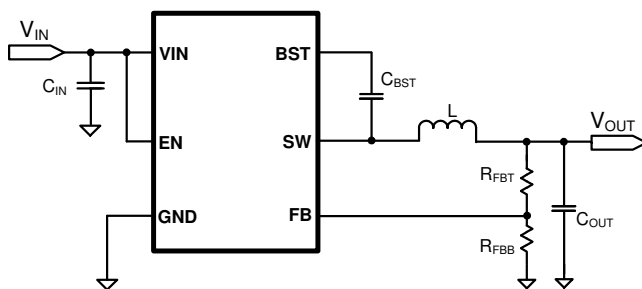
Simplified Schematic
