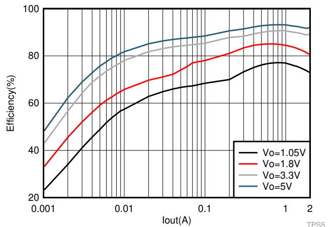
TPS562231 Efficiency
