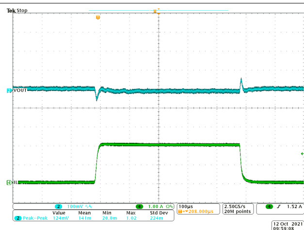
Figure 8-13. Transient Response 0 to 2 A with Slew Rate of 2.5 A/ \mu\text{s} (FCCM)
