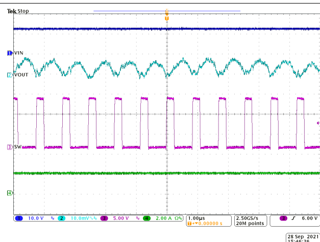
Figure 8-9. Steady State Waveforms, I_{OUT} = 2\text{ A}
