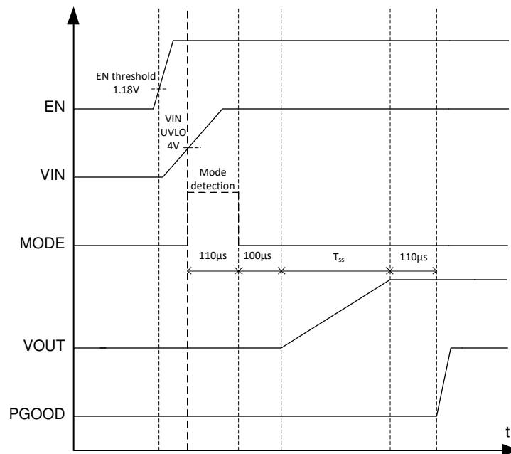
Figure 7-1. Power-Up Sequence
