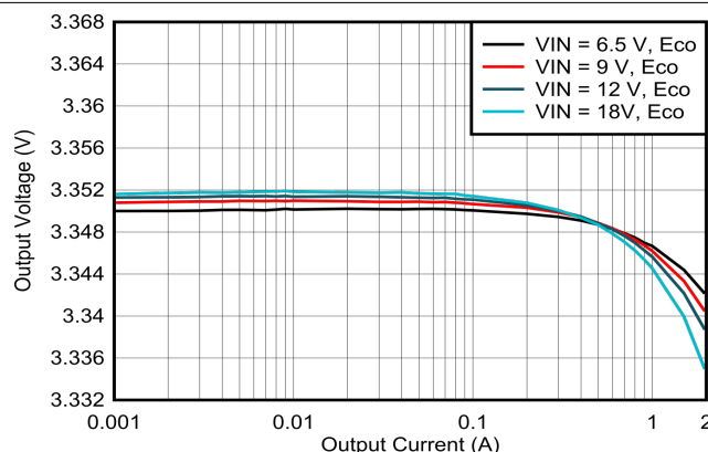
Figure 8-3. Load Regulation
