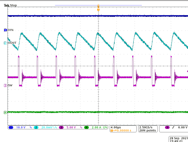
Figure 8-7. Steady State Waveforms, I_{OUT} = 0.1\text{ A}
