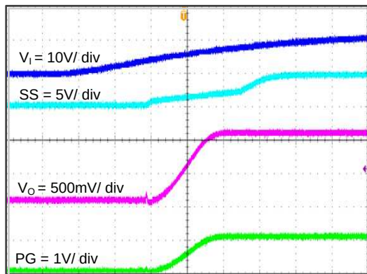
Time = 1 msec / div Figure 43. TPS563210A Start Up Relative To V_I
