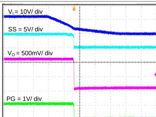
Time = 5 msec / div Figure 45. TPS563210A Shut Down Relative To V_I
