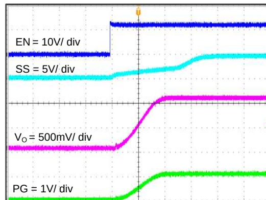
Time = 1 msec / div Figure 44. TPS563210A Start Up Relative To EN
