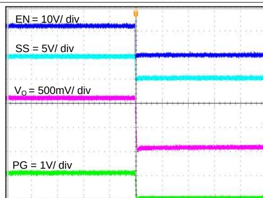
Time = 5 msec / div Figure 46. TPS563210A Shut Down Relative To EN
