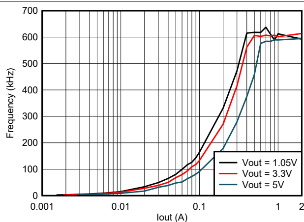
Figure 5-8. TPS562203 Frequency vs Loading
