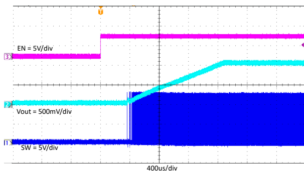
Figure 7-12. TPS562203 Enable On With 2A Loading
