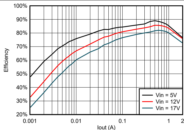
Figure 5-10. TPS562203 Efficiency at 0.6 Vout With 1.5uH Inductor
