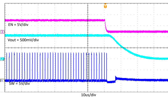
Figure 7-13. TPS562203 Enable Off With 2A Loading
