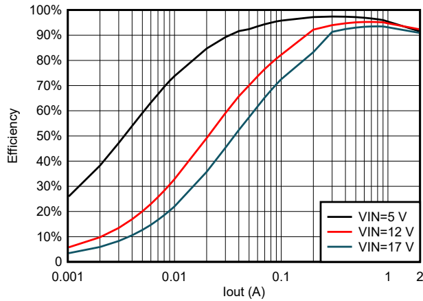
Figure 5-15. TPS562206 Efficiency at 3.3 Vout With 4.7uH Inductor
