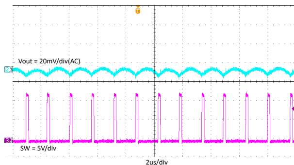
Figure 7-10. TPS562203 Output Voltage Ripple With 2A Loading
