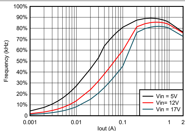
Figure 5-11. TPS562206 Efficiency at 0.6 Vout With 1.5uH Inductor
