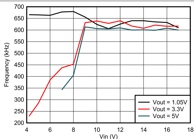
Figure 5-7. Frequency vs Input Voltage at 2A Loading
