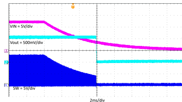
Figure 7-17. TPS562203 Power Off With 2A Loading
