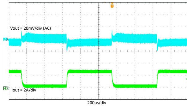
Figure 7-20. TPS562203 Load Transient With 0A to 2A
