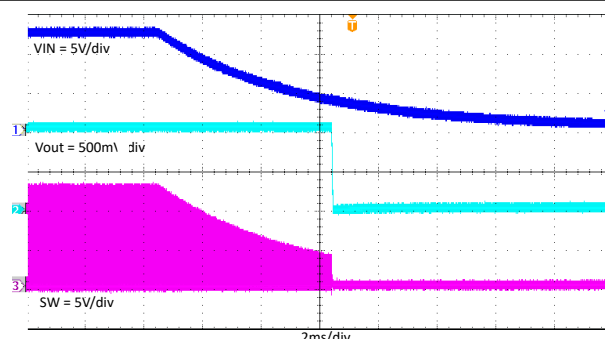
Figure 7-19. TPS562206 Power Off With 2A Loading
