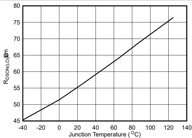
Figure 5-5. Low-Side R_{dson}
