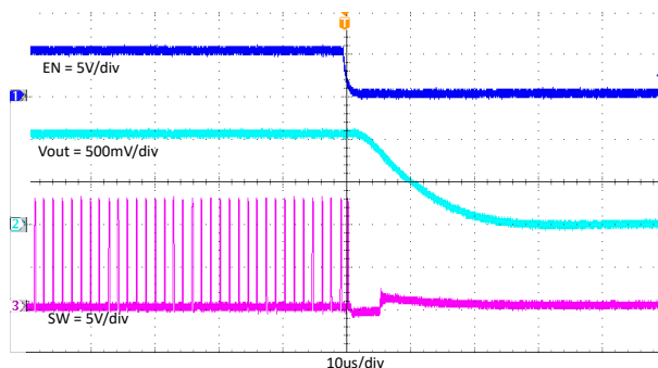
Figure 7-15. TPS562206 Enable Off With 2A Loading
