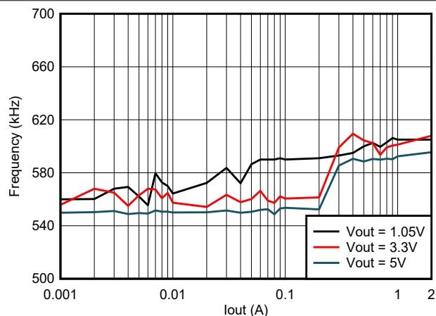
Figure 5-9. TPS562206 Frequency vs Loading
