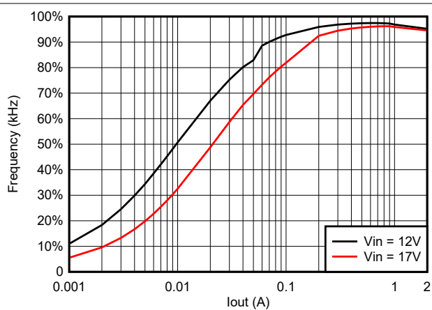
Figure 5-19. TPS562206 Efficiency at 7 Vout With 6.8uH Inductor
