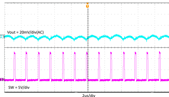
Figure 7-11. TPS562206 Output Voltage Ripple With 2A Loading
