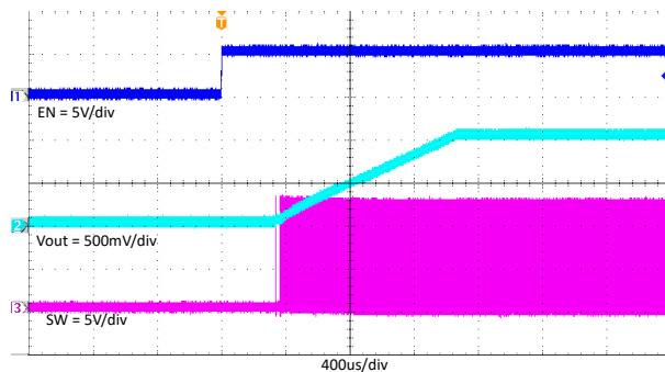
Figure 7-14. TPS562206 Enable On With 2A Loading
