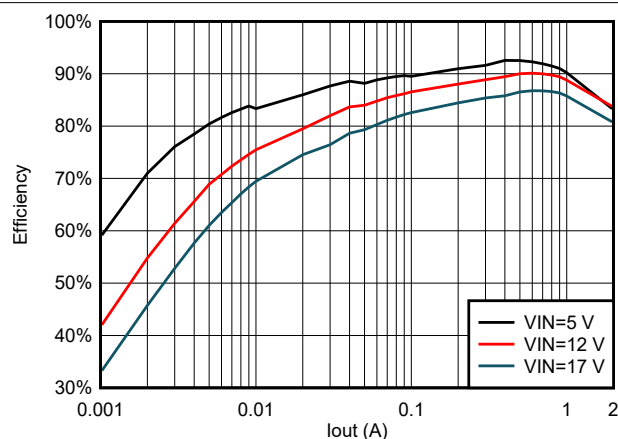
Figure 5-12. TPS562203 Efficiency at 1.05 Vout With 2.2uH Inductor
