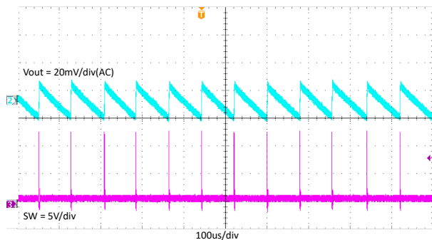
Figure 7-8. TPS562203 Output Voltage Ripple With 0.1A Loading
