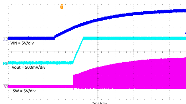
Figure 7-18. TPS562206 Power On With 2A Loading
