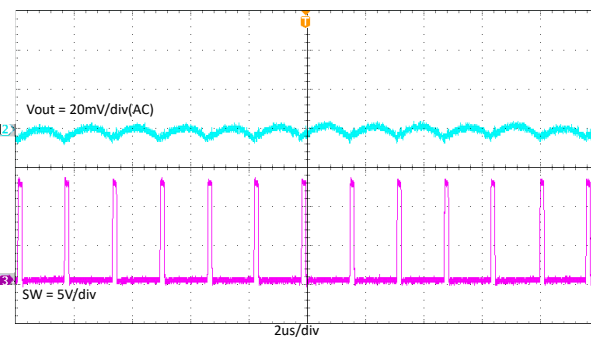
Figure 7-9. TPS562206 Output Voltage Ripple With 0.1A Loading
