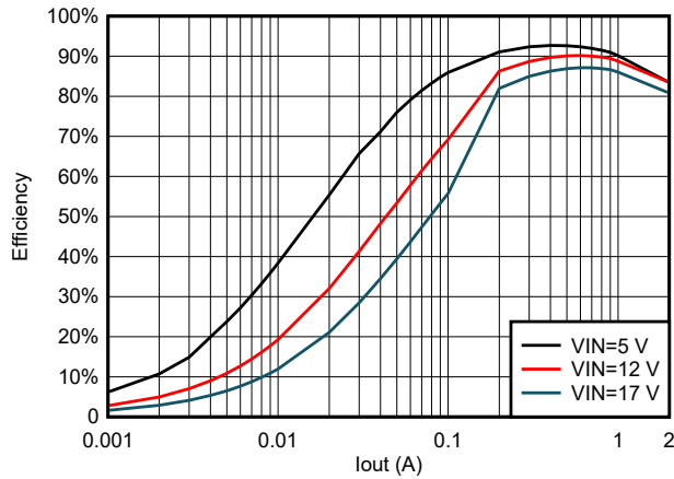
Figure 5-13. TPS562206 Efficiency at 1.05 Vout With 2.2uH Inductor
