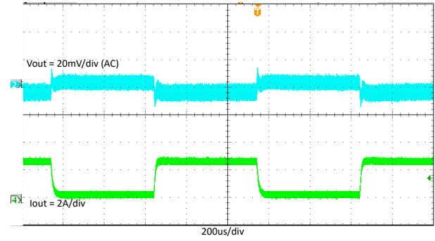
Figure 7-21. TPS562206 Load Transient With 0A to 2A
