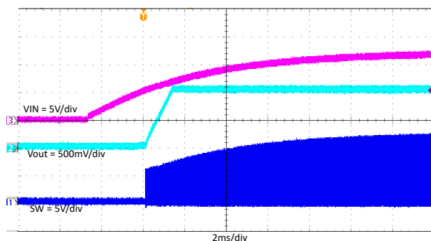
Figure 7-16. TPS562203 Power On With 2A Loading
