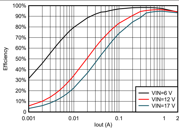
Figure 5-17. TPS562206 Efficiency at 5 Vout With 4.7uH Inductor
