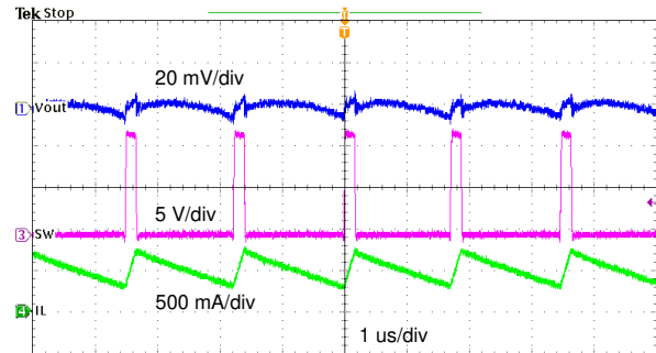
Figure 8-9. TPS561201 Output Voltage Ripple, I_{OUT} = 1\text{ A}
