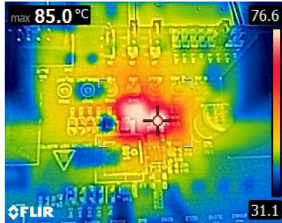
Figure 5-7. Thermal Image – 5V Output, TPS54KB20EVM, 6 Layers
