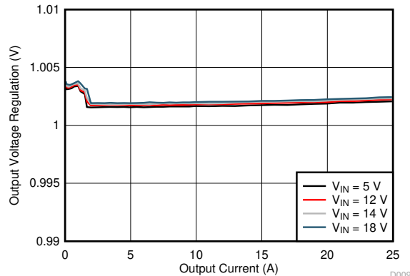
Figure 8-3. Output Voltage Regulation vs. Output Current
