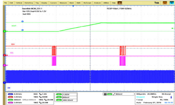
Figure 8-5. VOUT Command
