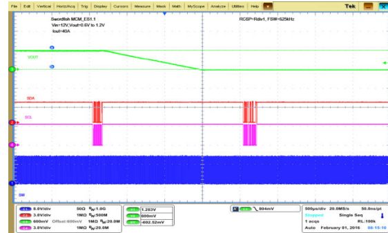
Figure 8-6. VOUT Command
