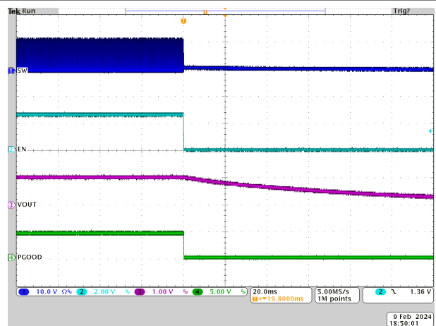
Figure 7-13. ENABLE Shutdown Waveform, PVIN = 12V, VOUT = 1.1V
