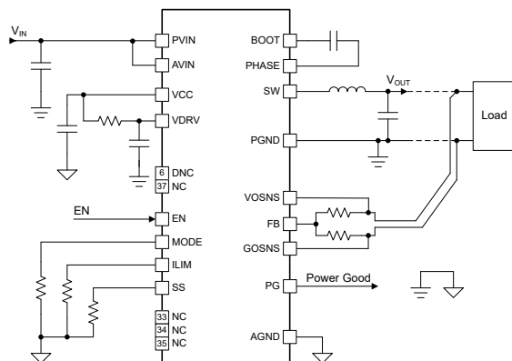
Simplified Schematic
