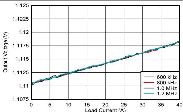
Figure 7-9. Load Regulation vs Output Current
