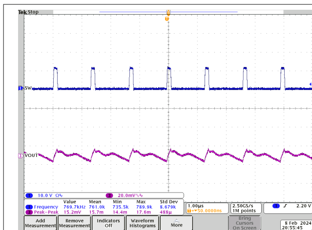
Figure 7-14. Output Voltage Ripple, 800kHz FCCM, 40A Load, PVIN = 12V, VOUT = 1.1V
