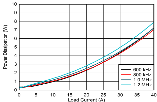
Figure 7-3. Power Dissipation vs Output Current
