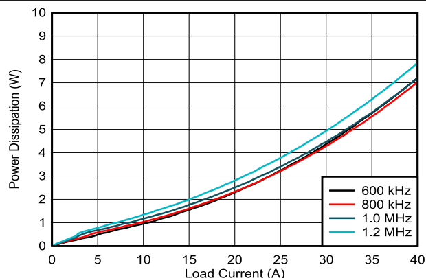
Figure 7-5. Power Dissipation vs Output Current
