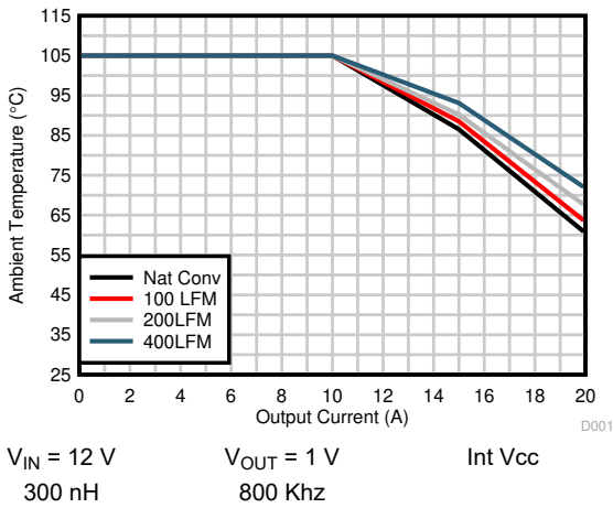
Figure 6-3. Safe Operating Area, V_{OUT} = 1.0\text{ V}
