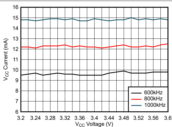
Figure 8-13. ICC Current vs External VCC Voltage
