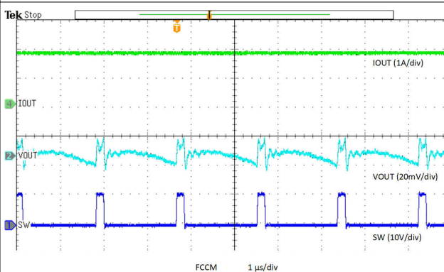
Figure 6-16. V OUT Ripple, FCCM, 20-A Load
