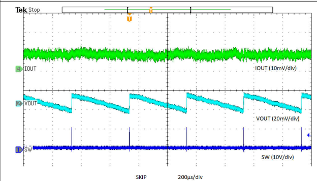
Figure 6-18. V OUT Ripple, Skip Mode, 10-mA Load
