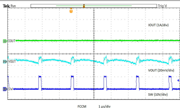
Figure 8-21. Output Voltage Ripple, FFCM, 0-A Load
