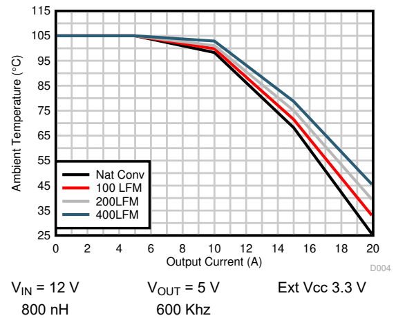
Figure 6-6. Safe Operating Area, V_{OUT} = 5\text{ V}
