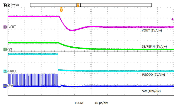
Figure 8-26. Overtemperature Protection in FCCM
