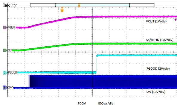
Figure 8-27. Exiting Overtemperature Protection in FCCM
