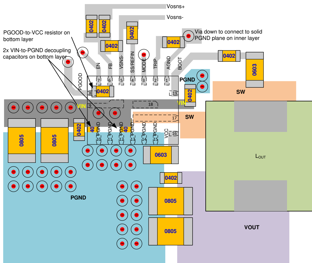
Figure 10-1. Layout Recommendation
