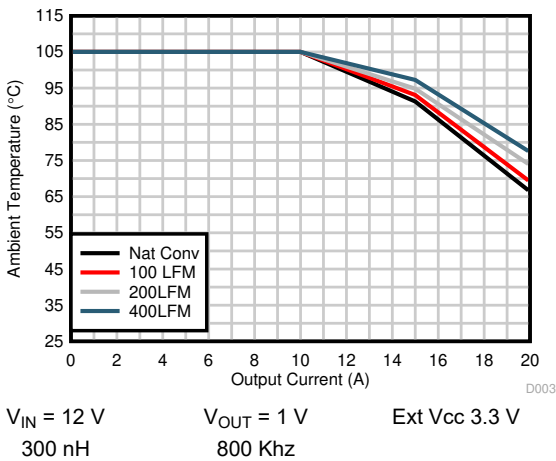
Figure 6-5. Safe Operating Area, V_{OUT} = 1\text{ V}
