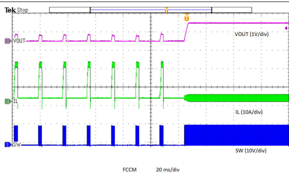
Figure 8-29. Hiccup Overcurrent
