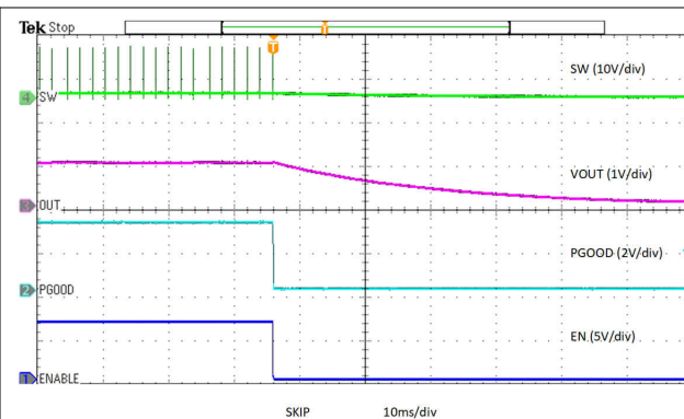
Figure 6-14. Enable Power Down, Skip
