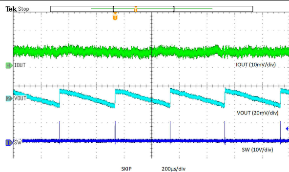
Figure 8-24. Output Voltage Ripple, Skip, 0.01-A Load
