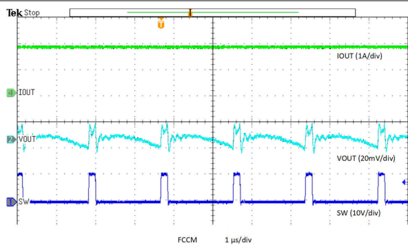
Figure 8-23. Output Voltage Ripple, FFCM, 20-A Load
