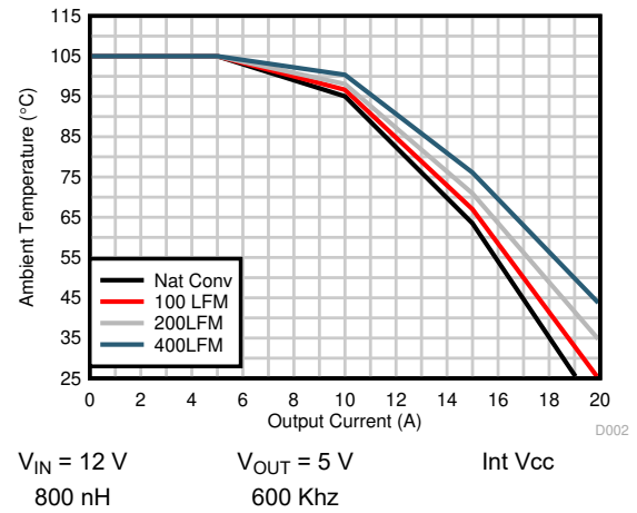
Figure 6-4. Safe Operating Area, V_{OUT} = 5\text{ V}
