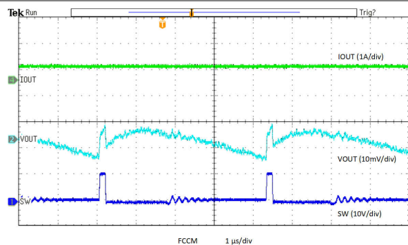
Figure 8-22. Output Voltage Ripple, FFCM, 0.5-A Load
