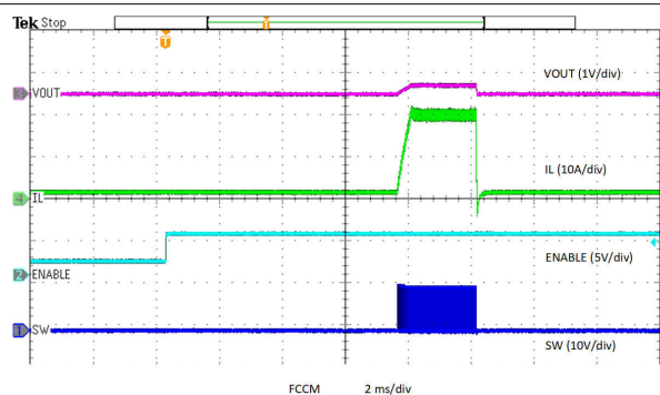
Figure 8-28. Enabled into Overcurrent
