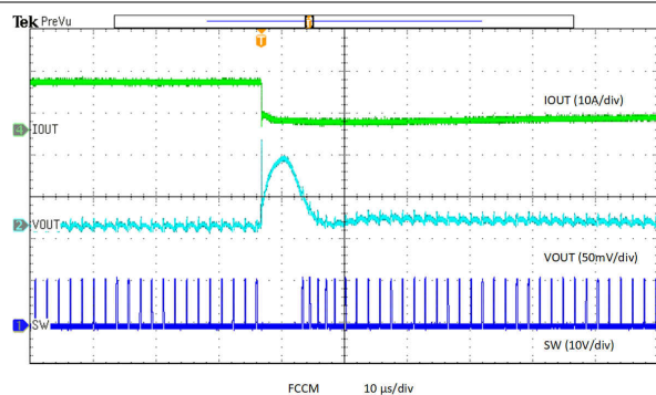
Figure 8-20. Unload Transient
