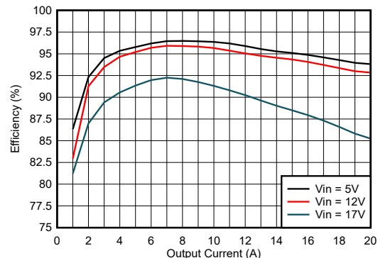
Typical Application Efficiency ( V_{IN} = 12V , external V_{CC} = 3.3V , FCCM, F_{sw} = 800kHz , DCR = 1.4m\Omega )
