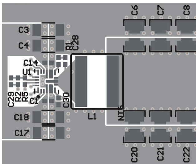
Figure 8-2. Layout Recommendation
