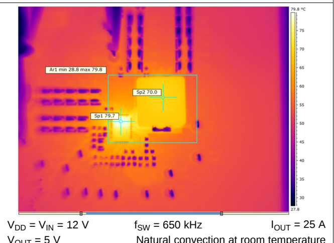
Figure 12. Thermal Image
