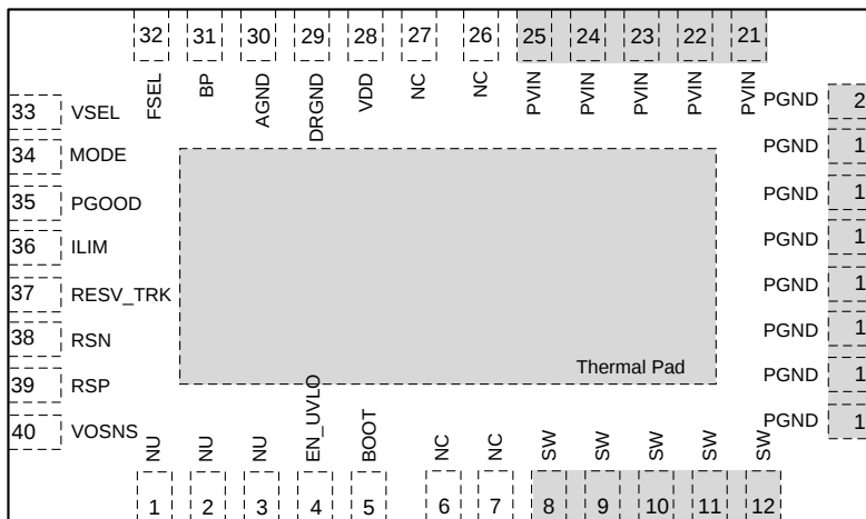
Pin Functions
