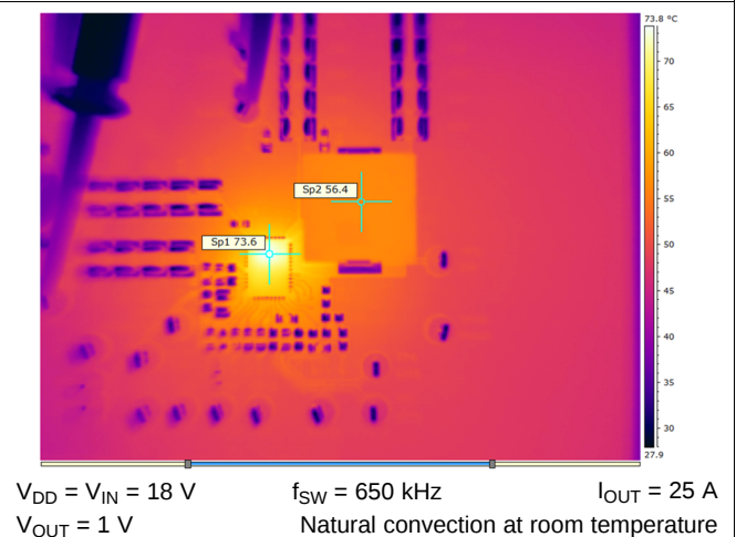
Figure 10. Thermal Image
