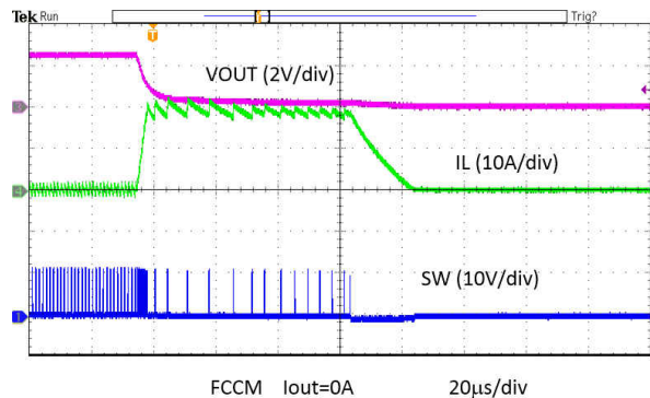
Figure 8-32. Overcurrent Protection
