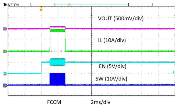
Figure 8-33. Enabled into Overcurrent
