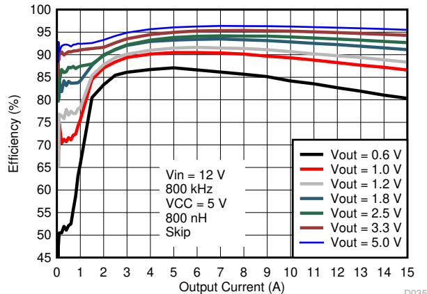
Figure 8-3. Efficiency vs Output Current, VCC = 5.0V External VCC Bias
