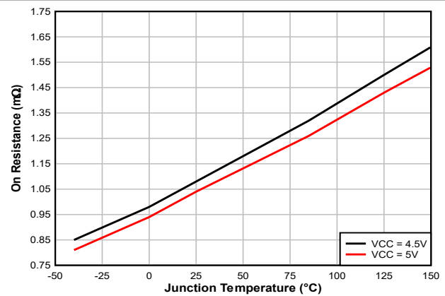
Figure 5-4. Low-Side MOSFET On-Resistance ( R_{DS(on)} ) vs Junction Temperature
