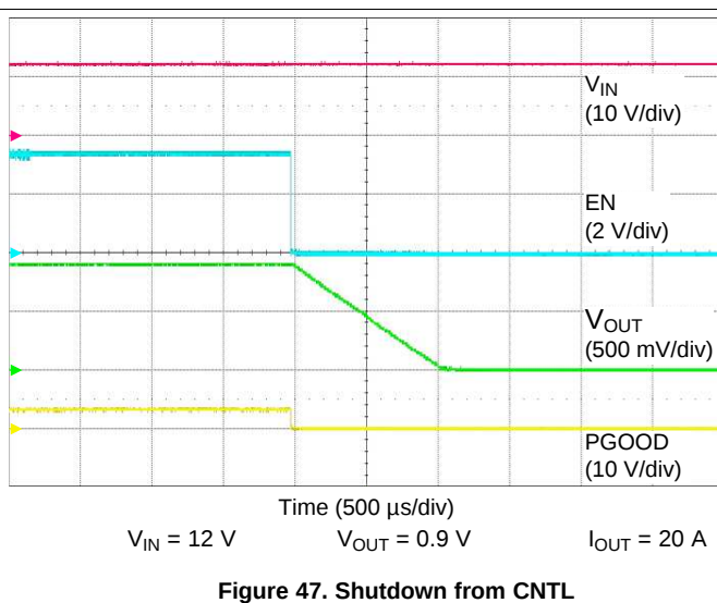
Figure 47. Shutdown from CNTL
