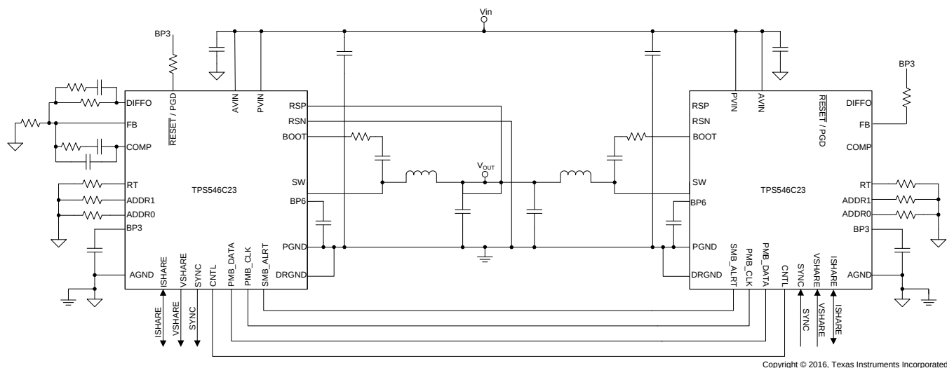
Figure 23. 2-Phase Application
