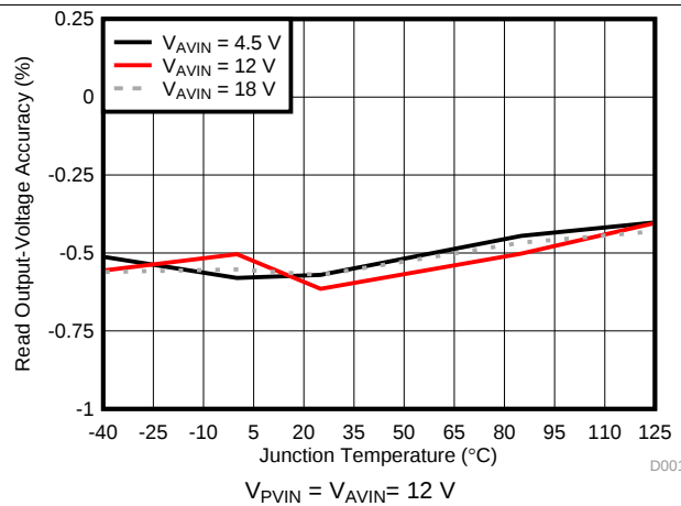
Figure 16. READ_VOUT Accuracy vs Junction Temperature
