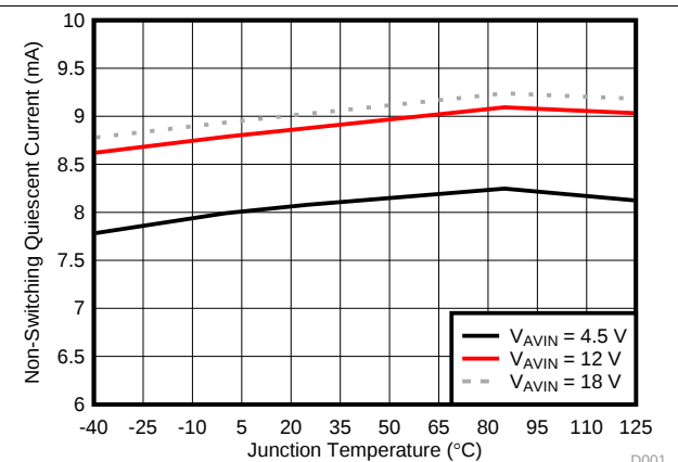
Figure 9. Non-Switching Input Current ( I_{AVIN} ) vs Junction Temperature
