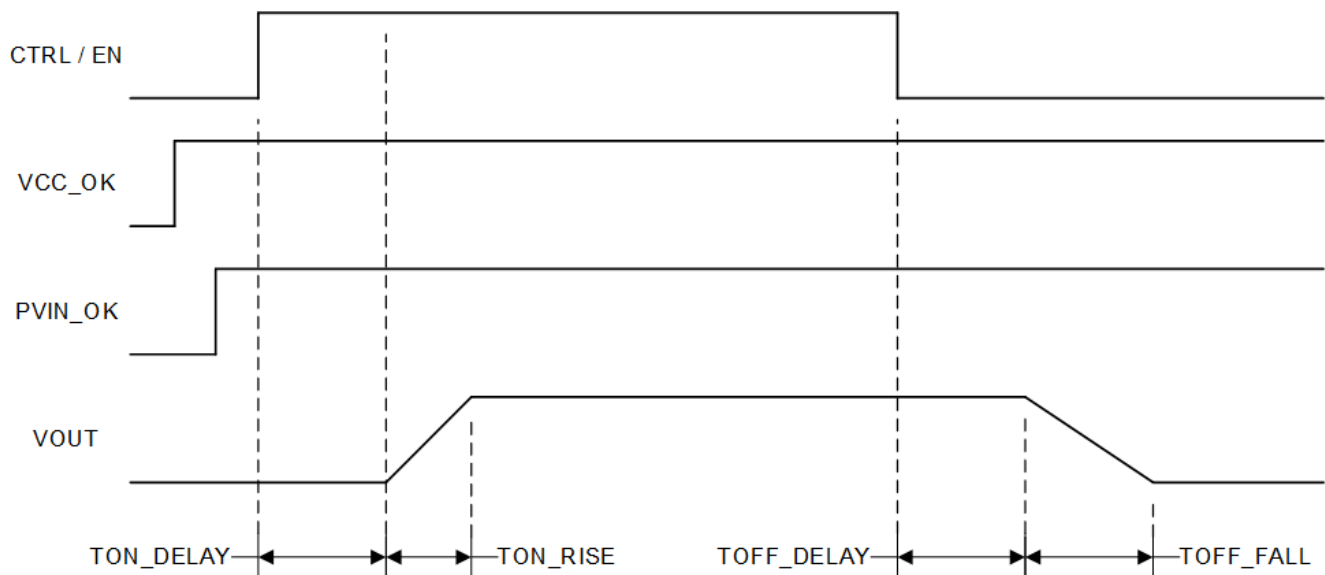
Figure 6-4. TPS546B25W Start-Up and Shutdown
