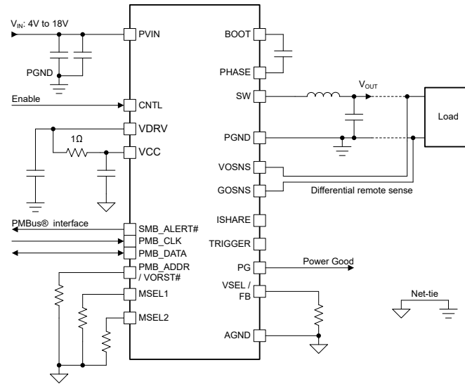
Simplified Schematic
