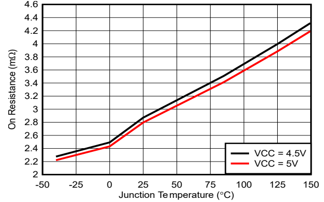
Figure 5-2. High-Side MOSFET On-Resistance ( R_{DS(on)} ) vs Junction Temperature
