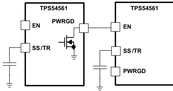
Figure 7-4. Schematic for Sequential Start-Up Sequence
