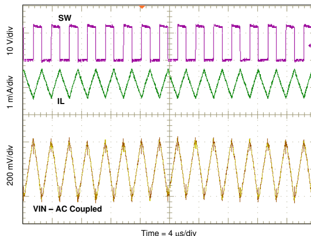
Figure 8-13. Input Ripple CCM
