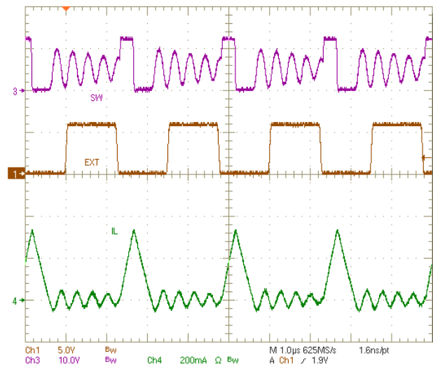
Figure 7-14. Plot of Synchronizing in DCM
