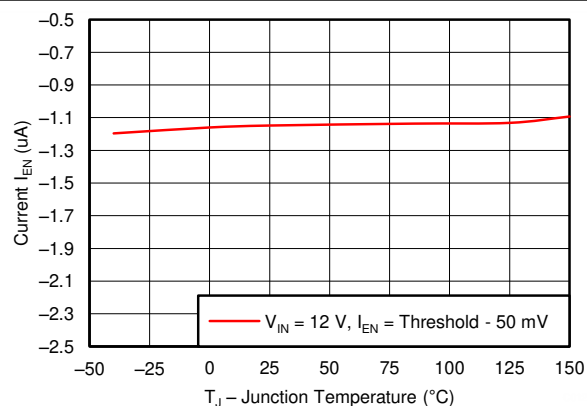
Figure 6-12. EN Pin Current vs Junction Temperature
