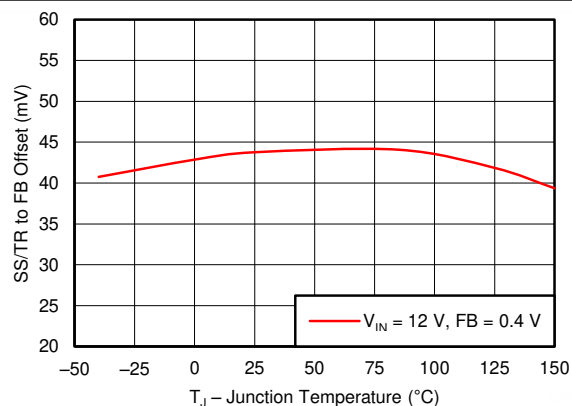
Figure 6-24. SS/TR to FB Offset vs Temperature
