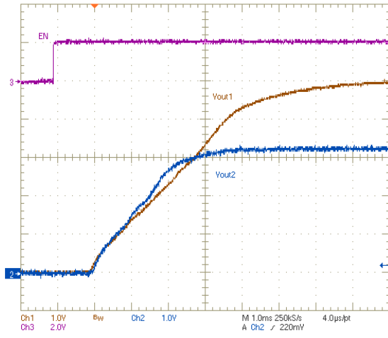
Figure 7-9. Ratio-Metric Startup with Tracking Resistors
