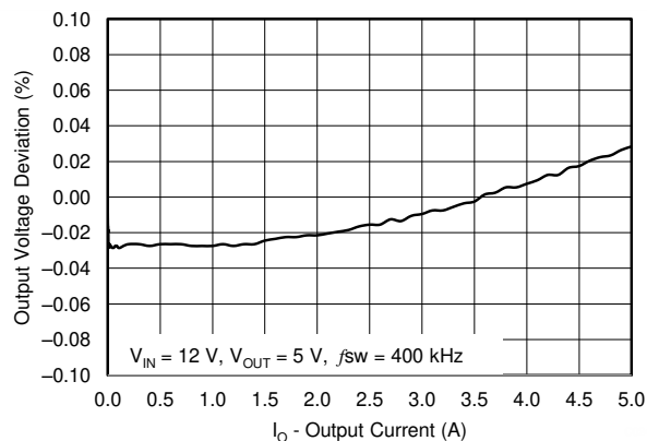
Figure 8-24. Regulation vs Load Current
