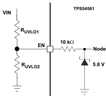
Figure 7-2. Internal EN Pin Clamp
