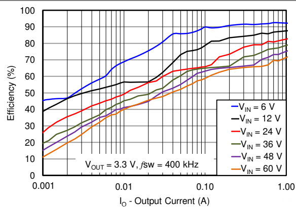
Figure 8-21. Light Load Efficiency
