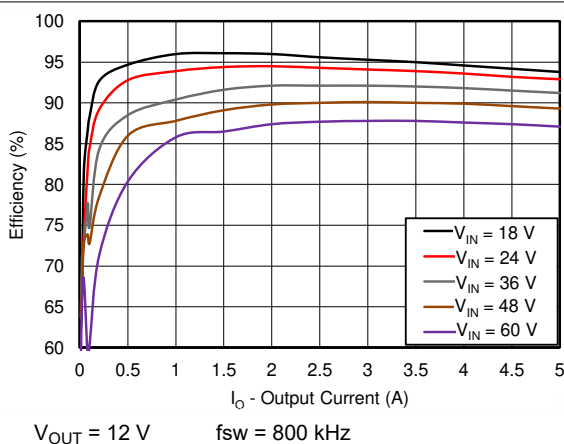
Figure 8-22. Efficiency vs Output Current
