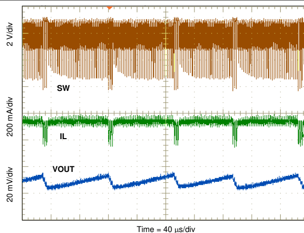
Figure 8-15. Low Dropout Operation
