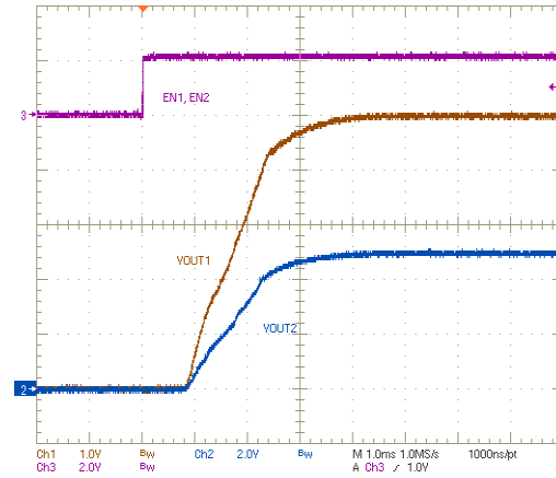
Figure 7-7. Ratio-Metric Startup using Coupled SS/TR pins
