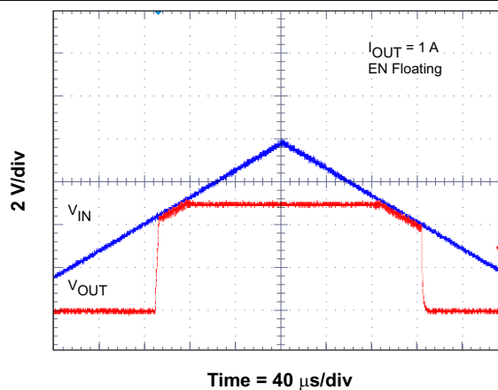
Figure 8-17. Low Dropout Operation
