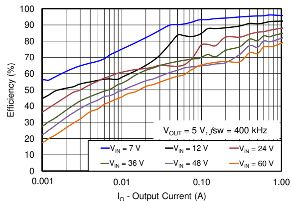
Figure 8-19. Light Load Efficiency
