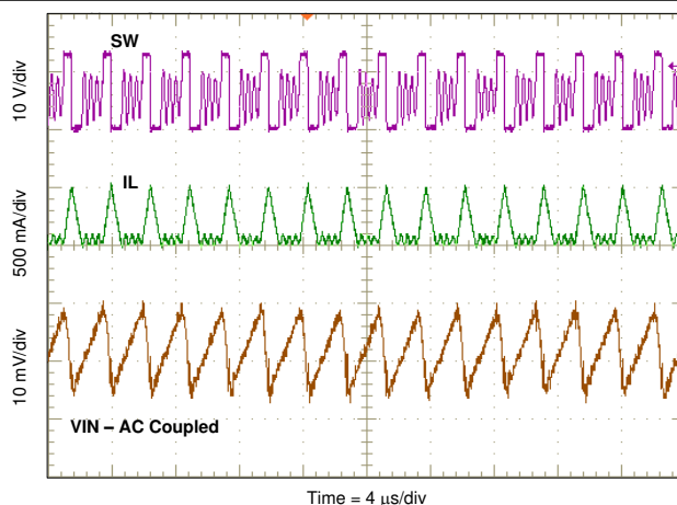
Figure 8-14. Input Ripple DCM
