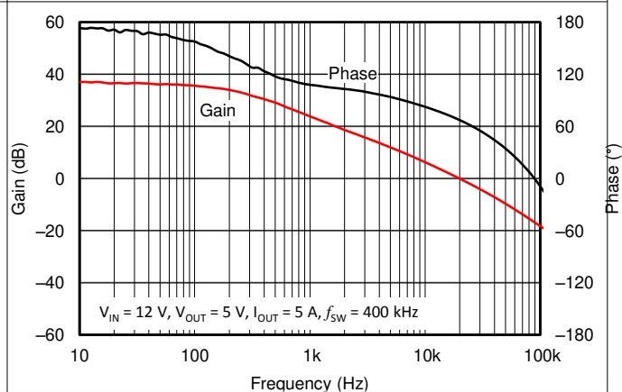
Figure 8-23. Overall Loop Frequency Response
