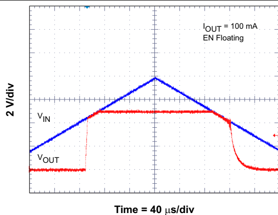
Figure 8-16. Low Dropout Operation
