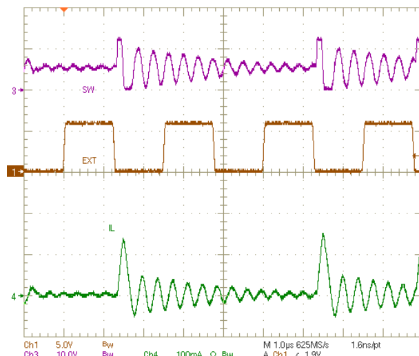
Figure 7-15. Plot of Synchronizing in Eco-mode
