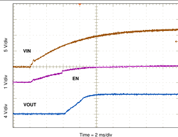
Figure 8-8. Start-up With VIN
