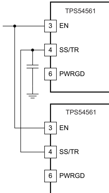
Figure 7-6. Schematic for Ratio-Metric Start-Up Sequence
