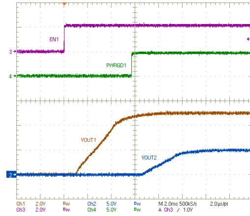
Figure 7-5. Sequential Startup using EN and PWRGD
