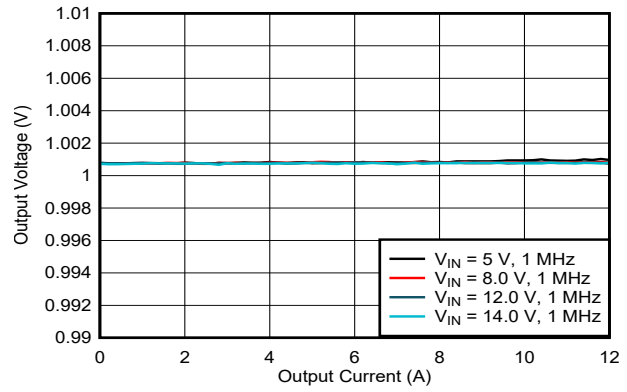
Figure 7-5. Load Regulation
