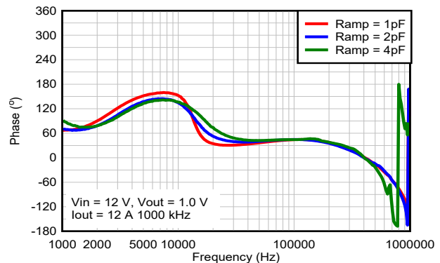
Figure 6-8. Loop Phase vs Ramp Settings
