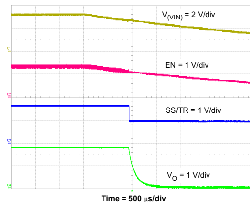
Figure 8-7. Power Down V_O , V_{(IN)}
