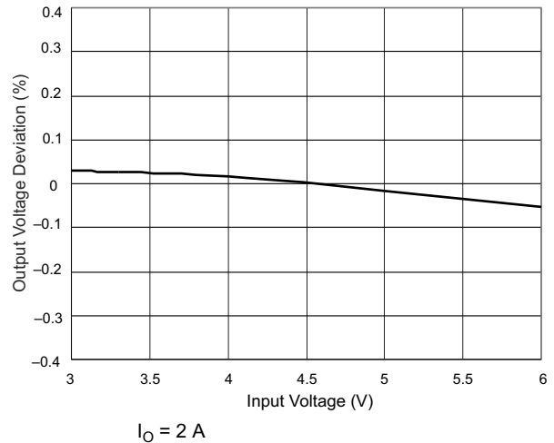
Figure 8-15. Regulation vs Input Voltage
