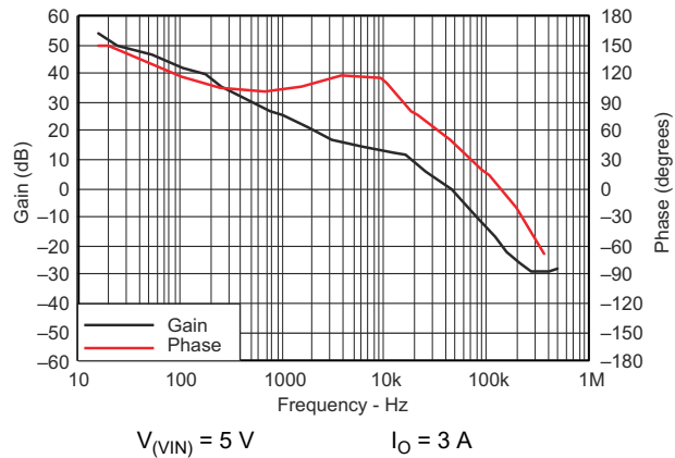
Figure 8-13. Closed-Loop Response
