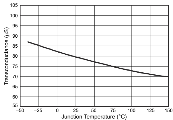
Figure 6-8. Transconductance (Slow Start) vs Junction Temperature
