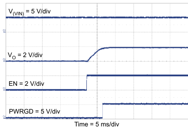
Figure 8-10. Power Up V_O , EN
