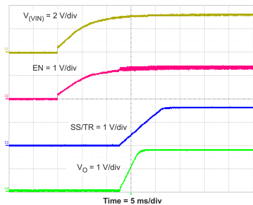
Figure 8-6. Power Up V_O , V_{(IN)}
