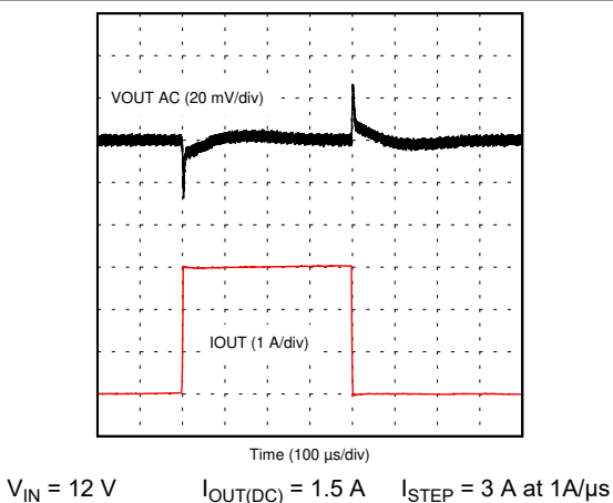
Figure 8-8. Load Transient
