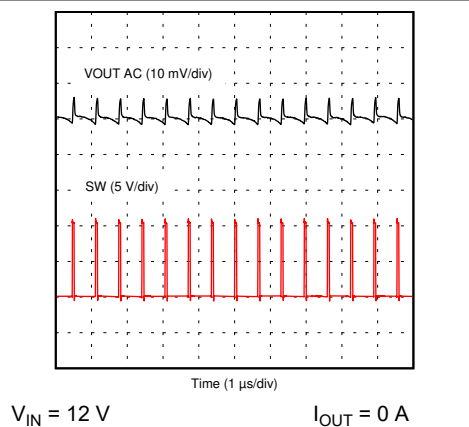
Figure 8-28. Output Ripple – No Load
