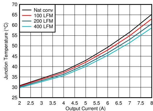
Figure 6-8. Junction Temperature vs Output Current – 3.3-V Output
