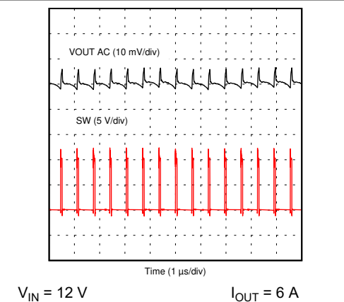
Figure 8-29. Output Ripple – 6-A Load
