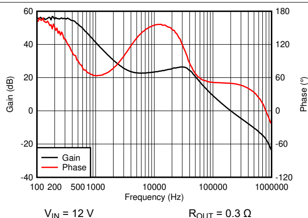
Figure 8-27. Bode Plot
