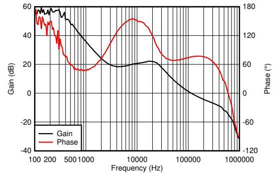
Figure 8-34. Bode Plot
