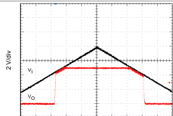
I O = 1 A EN floating Time = 40 μs/div
