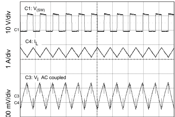
I O = 3.5 A Time = 2 μs/div
