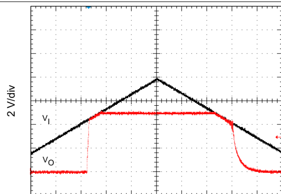
I O = 100 mA EN floating Time = 40 μs/div
