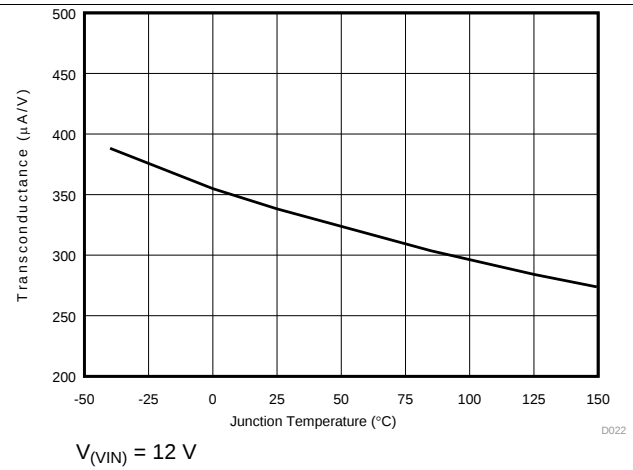
Figure 8. EA Transconductance vs Junction Temperature
