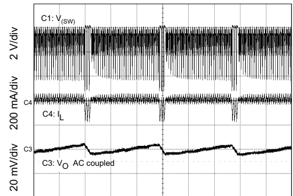
V I = 5.5 V V O = 5 V No load EN floating Time = 20 μs/div
