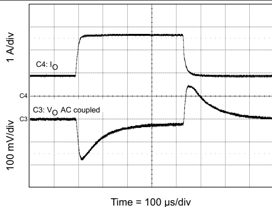
Figure 49. Load Transient
