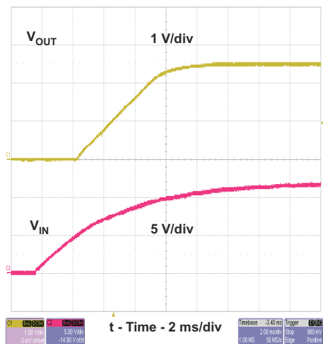
Figure 8-10. TPS54332 Start-Up
