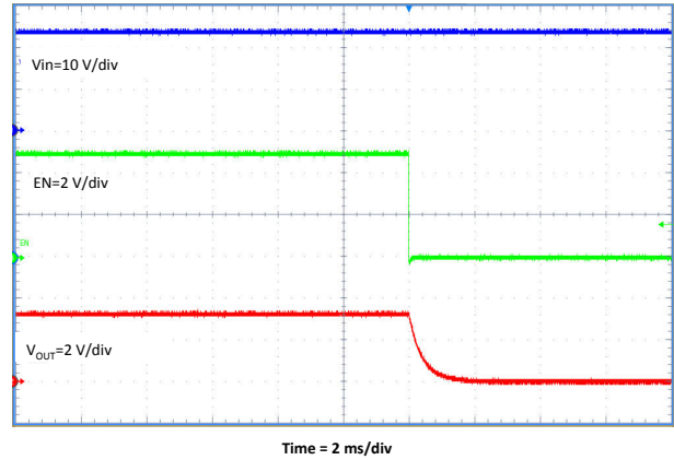
Figure 8-15. Shutdown Relative to EN
