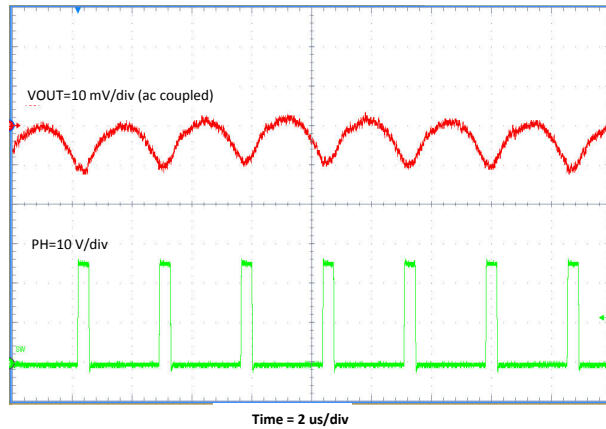
Figure 8-8. Output Voltage Ripple
