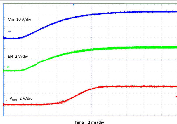
Figure 8-12. Start-Up Relative to VIN
