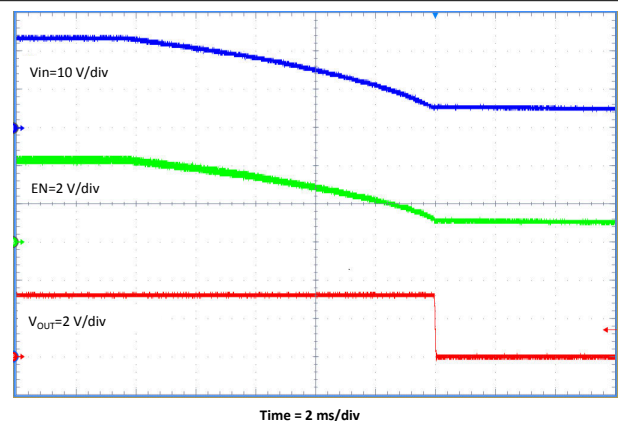
Figure 8-13. Shutdown Relative to VIN
