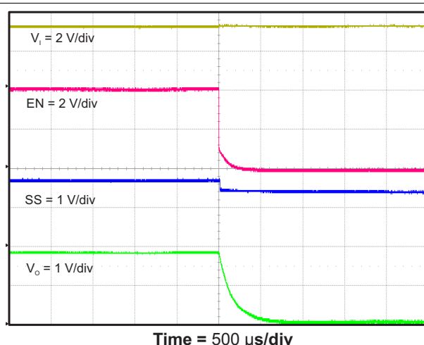
Figure 43. Power Down, V_{OUT} , V_{IN}
