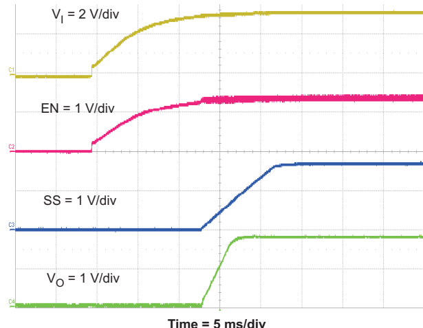
Figure 42. Power Up, V_{OUT} , V_{IN}
