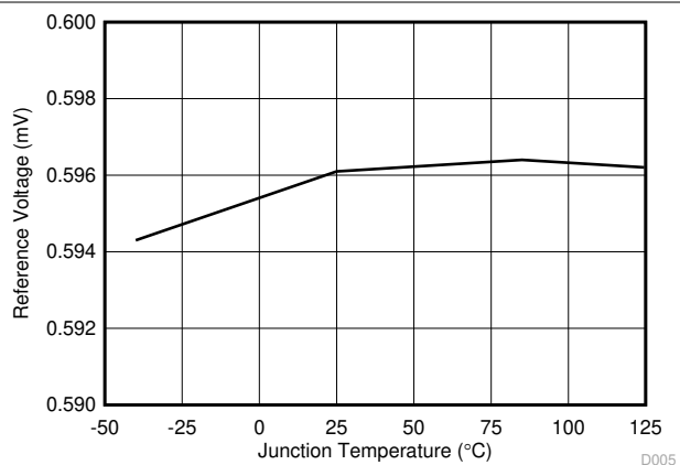
Figure 6-5. Reference Voltage vs Junction Temperature
