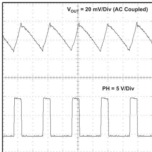
Figure 8-10. Output Voltage Ripple and PH Node, I_O = 3 \text{ A}
