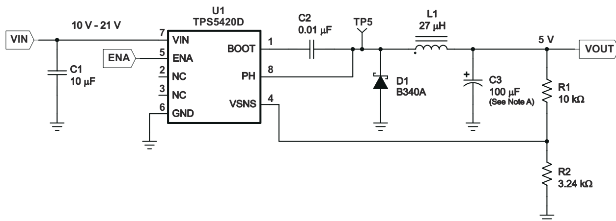
Figure 8-4. 10-V — 21-V Input to 5-V Output Application Circuit
